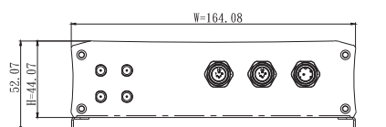
#M12 LAN/DC-in
