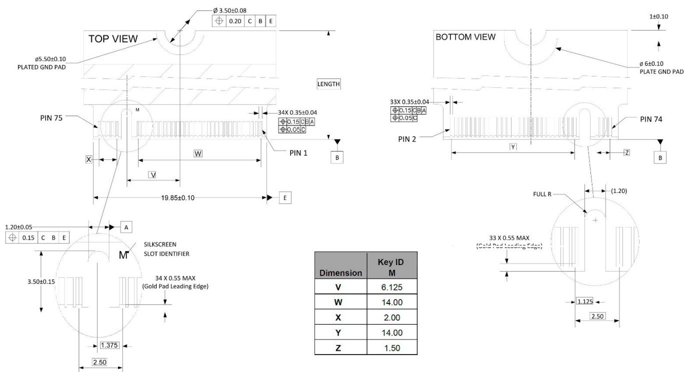
Figure 4: M.2 Connector Dimensions in mm
