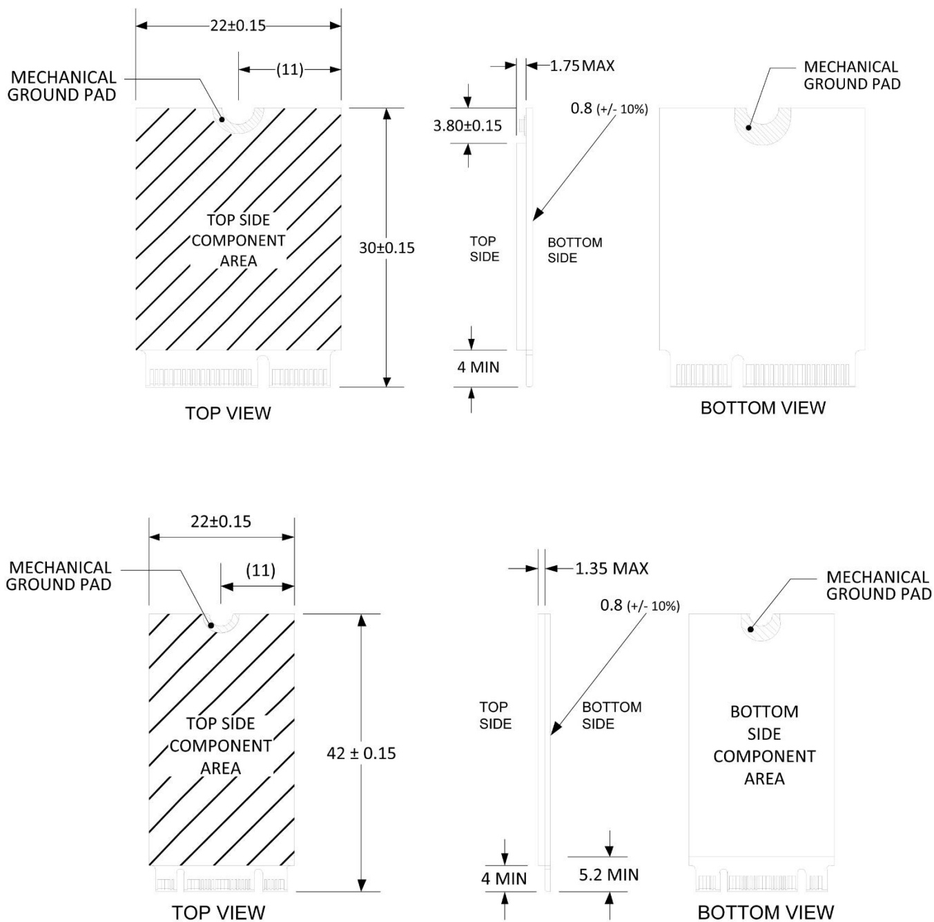
Figure 3: N-20m2 dimensions in mm
