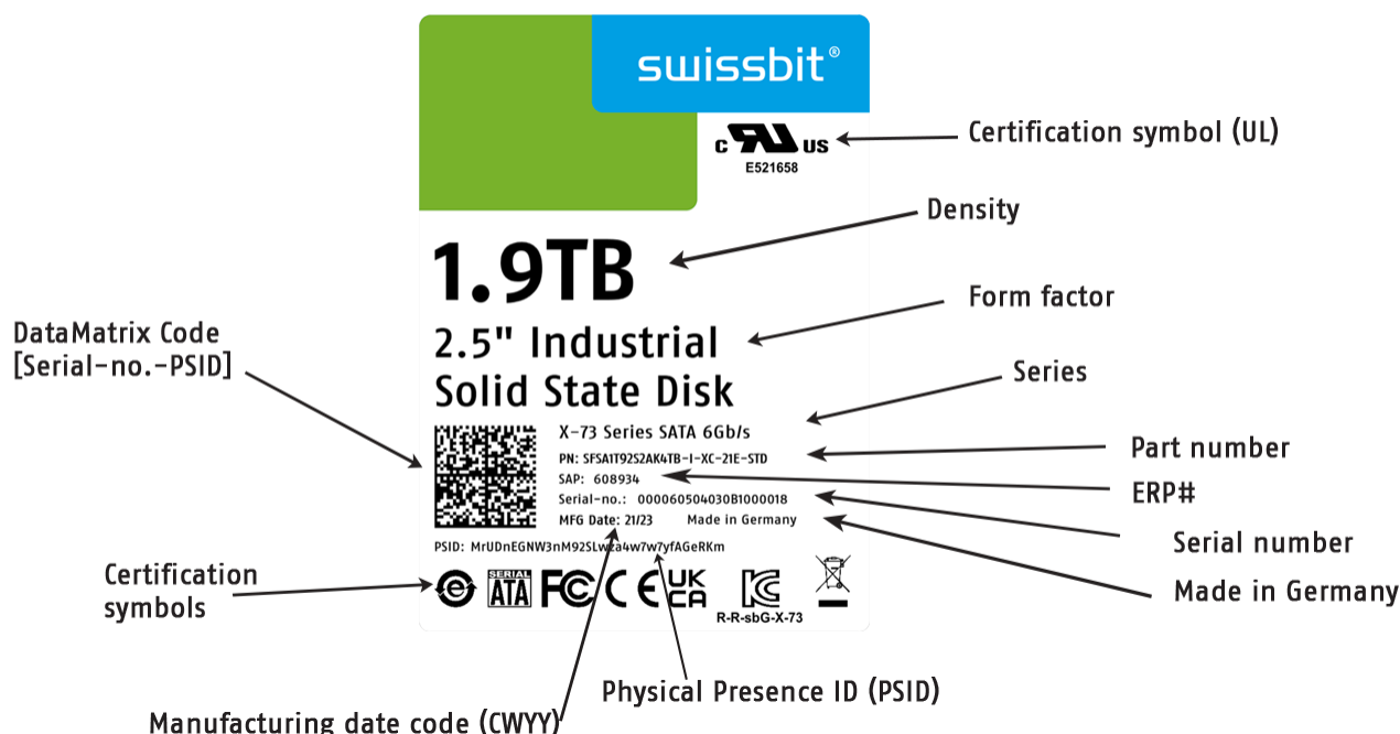
Figure 5: X-73 label details
