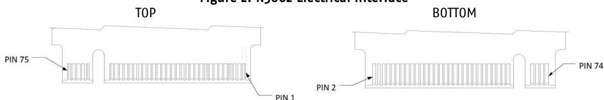
Figure 2: N3602 Electrical Interface
