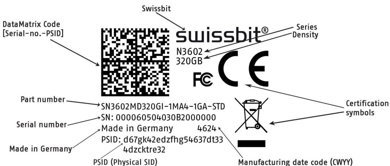
Figure 5: N3602 label details
