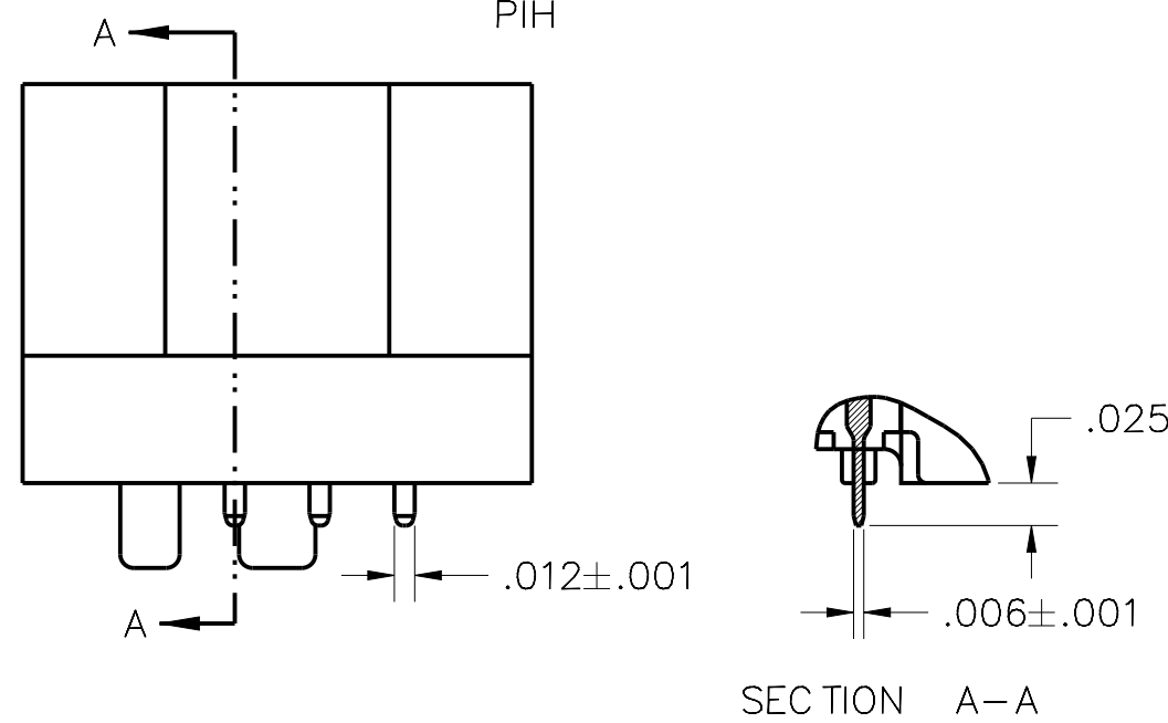
TERMINATION TYPE 01 PIH
