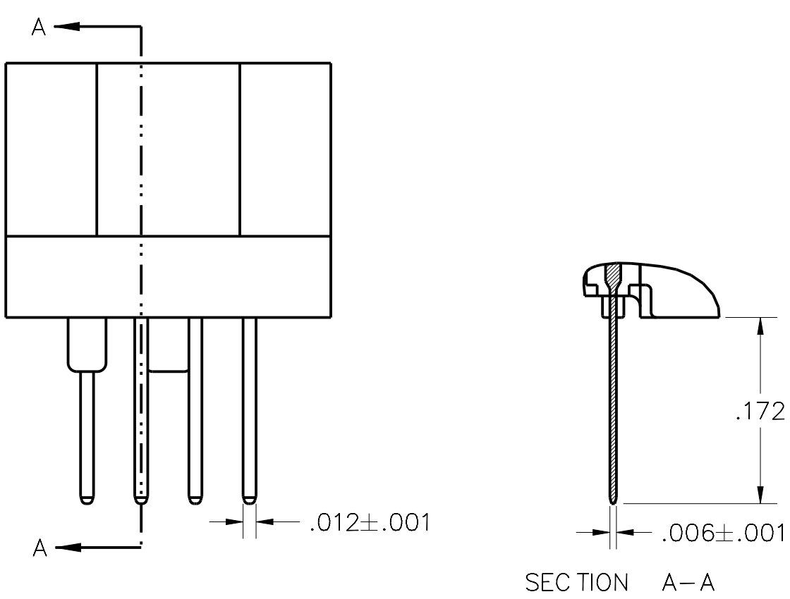
TERMINATION TYPE 06 PTH .172" LENGTH
