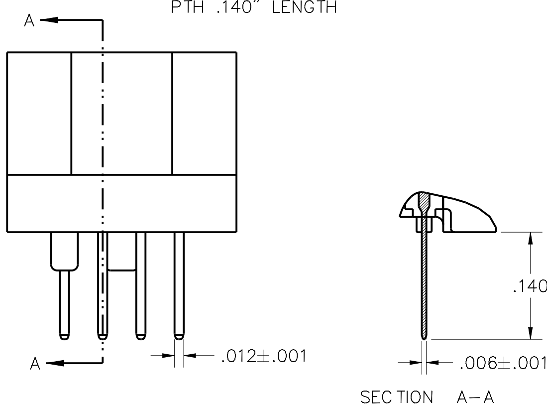
TERMINATION TYPE 04 PTH .140" LENGTH
