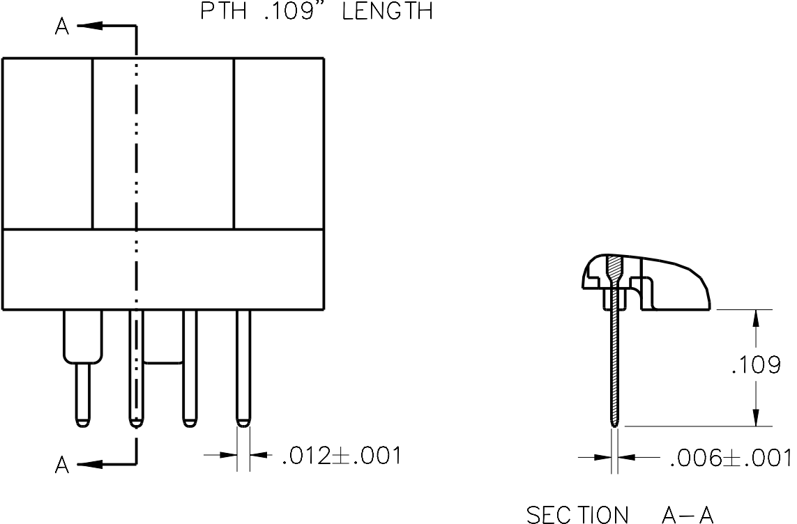
TERMINATION TYPE 03 PTH .109" LENGTH
