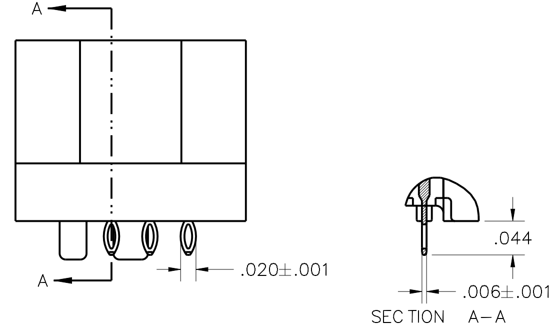
TERMINATION TYPE 00 PRESS-FIT
