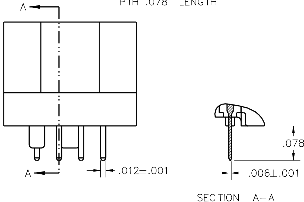
TERMINATION TYPE 02 PTH .078" LENGTH
