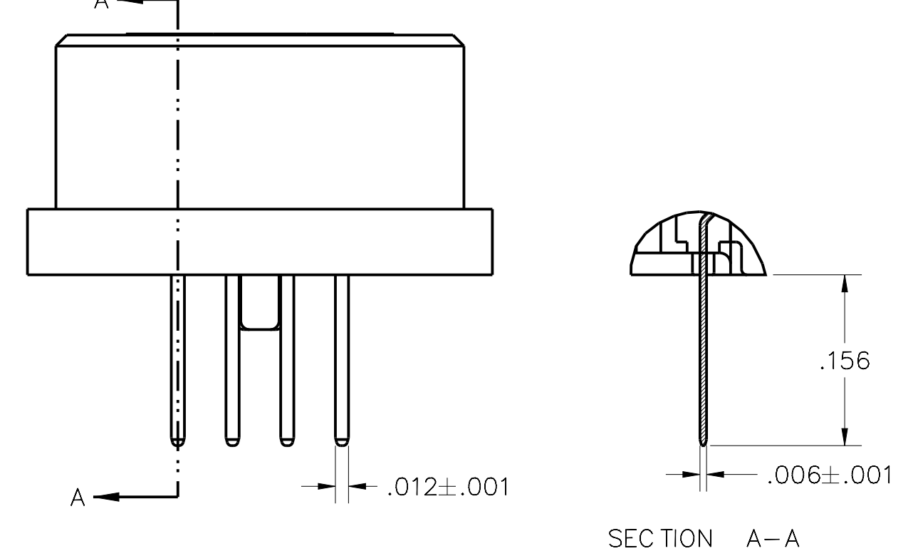
TERMINATION TYPE 05 PTH .156" LENGTH
