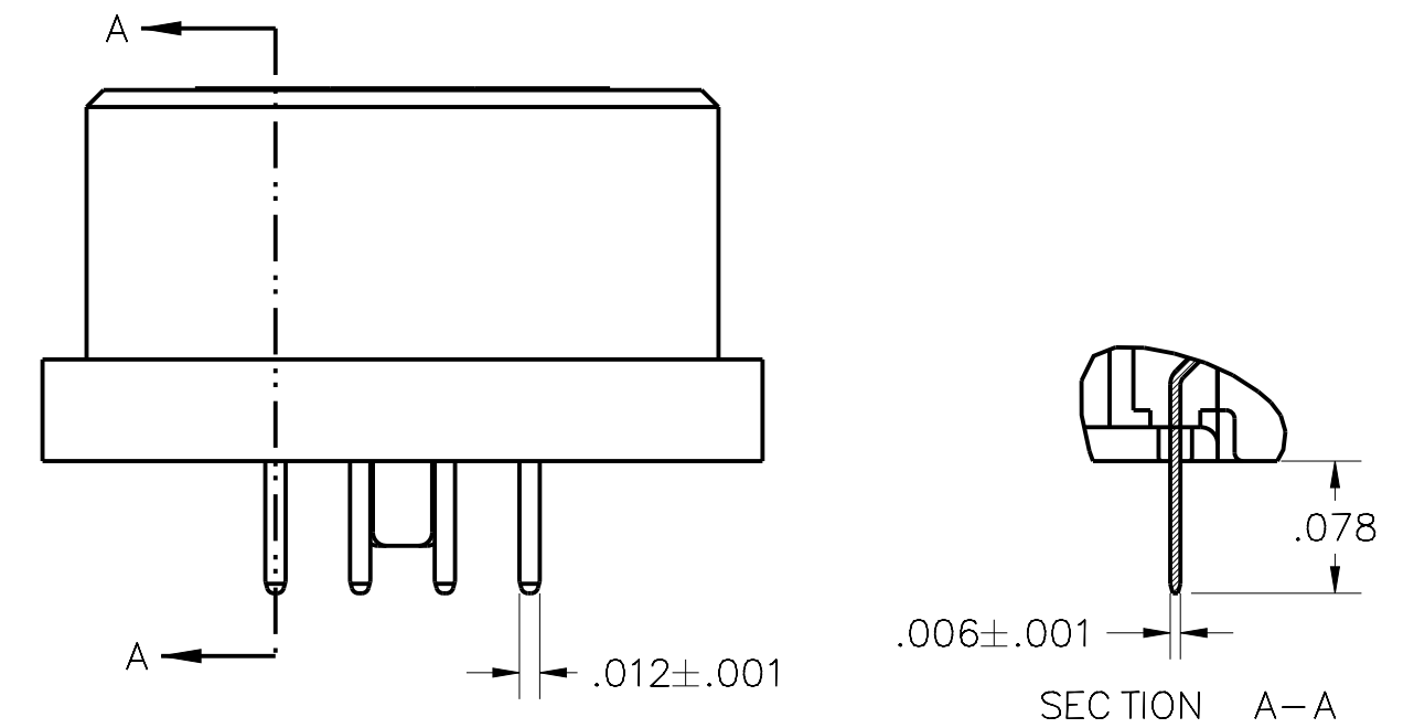
TERMINATION TYPE 02 PTH .078" LENGTH
