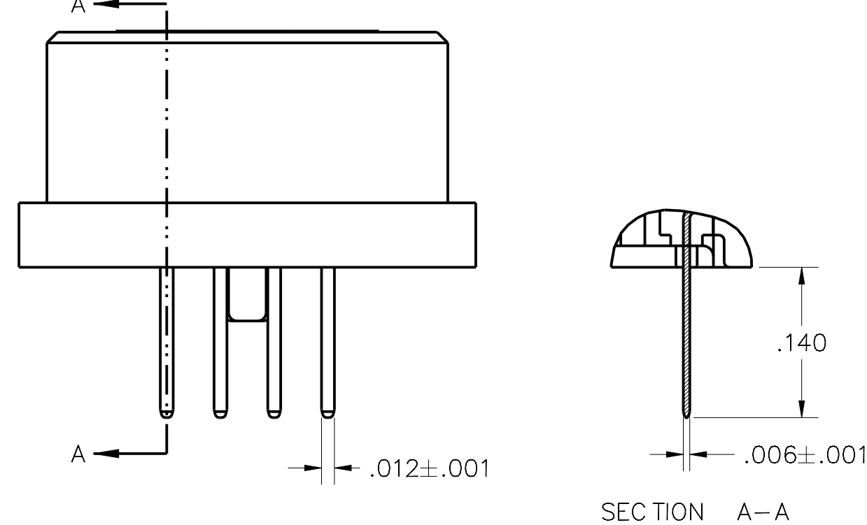
TERMINATION TYPE 04 PTH .140" LENGTH
