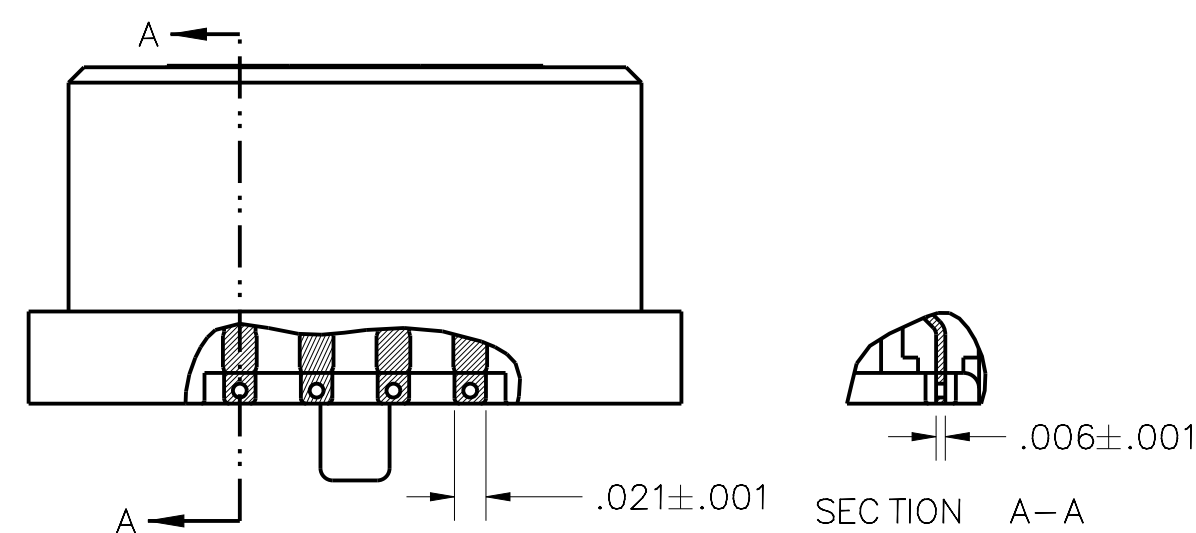
TERMINATION TYPE 10 & 11 SMT
