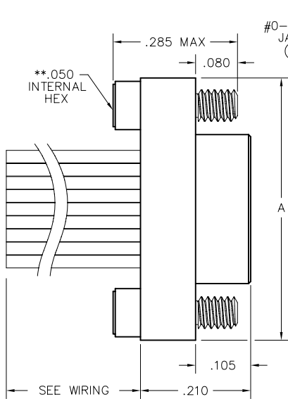
PLUG
