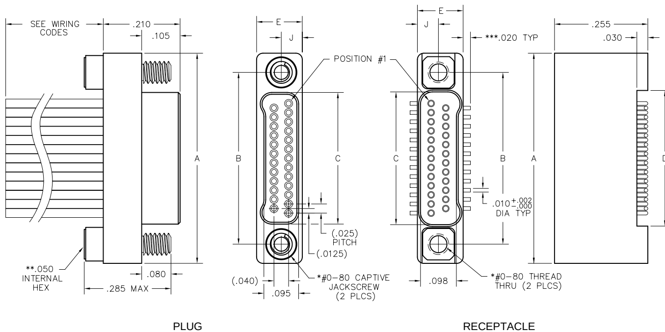
PLUG
