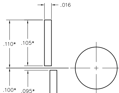
* = For .040" lead envelope, add .020" to noted dimensions
