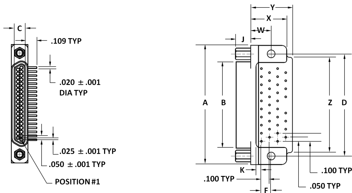
#2-56 JACKPOST (2 PLCS)
