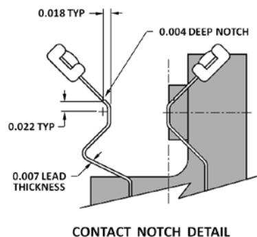
CONTACT NOTCH DETAIL
