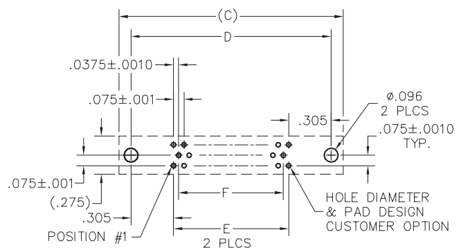
PCB LAYOU VIEWED FROM COMPONENT SIDE
