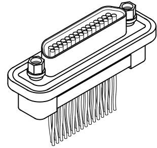
MM-2H2-031-261-26WA (RECEPTACLE)
