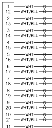
21 POSITION
