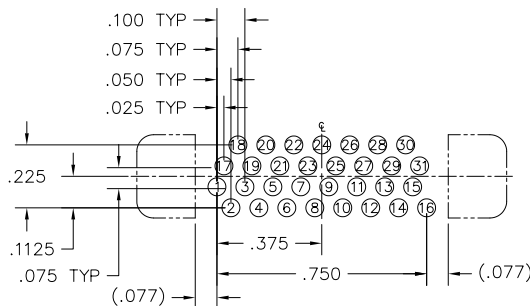
31 POSITION
