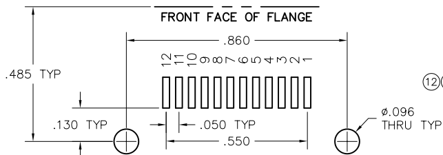
PLUG PC BOARD LAYOUT COMPONENT SIDE
