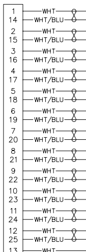
25 POSITION
