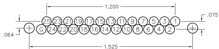
25 POSITION
