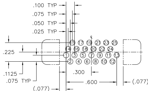
25 POSITION
