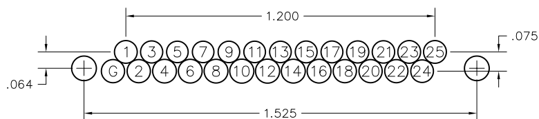
25 POSITION
