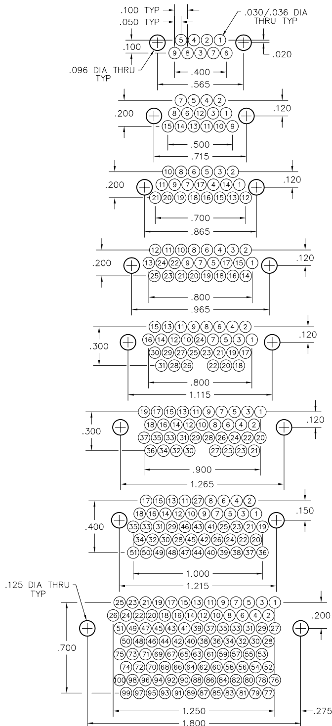
RECEPTACLE PC BOARD LAYOUT COMPONENT SIDE
