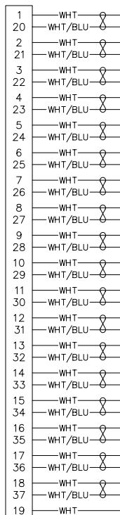
37 POSITION
