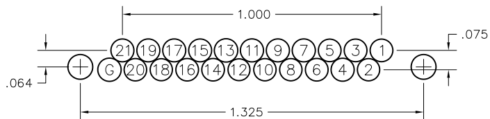
21 POSITION
