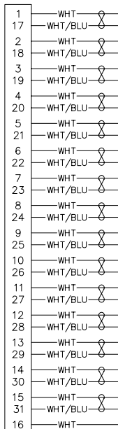
31 POSITION
