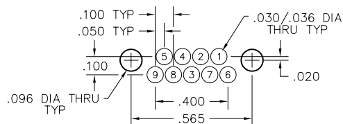
RECEPTACLE PC BOARD LAYOUT COMPONENT SIDE
