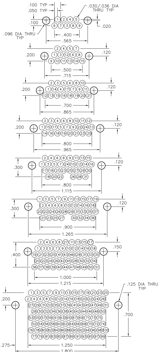
PLUG PC BOARD LAYOUT COMPONENT SIDE
