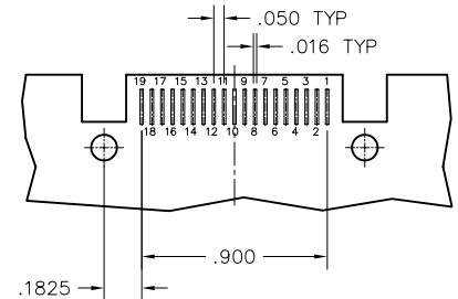
PLUG PC BOARD LAYOUT CIRCUIT SIDE
