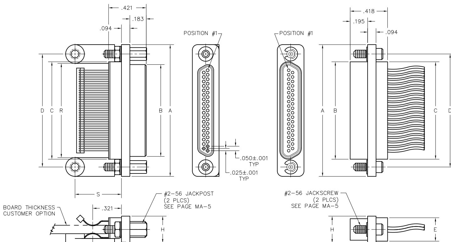
PLUG
