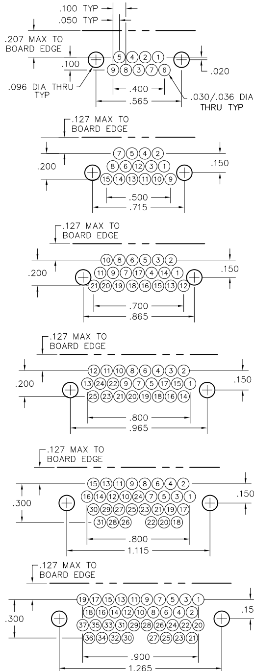
RECEPTACLE PC BOARD LAYOUT COMPONENT SIDE
