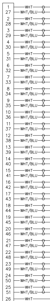
51 POSITION 2 rows
