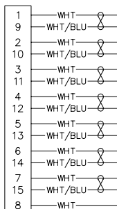
15 POSITION
