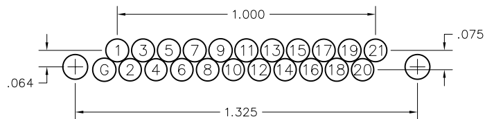
21 POSITION
