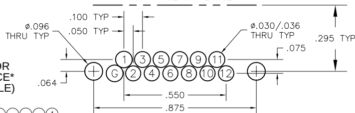
12 POSITION
