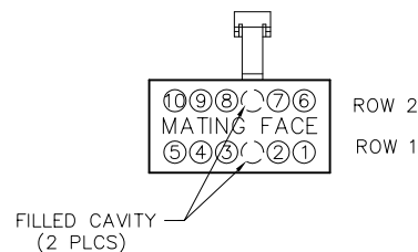
RECEPTACLE MA-241-010-261-ALCWA
