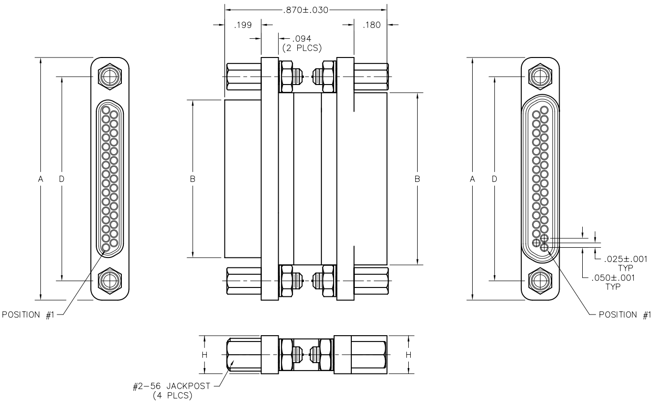
PLUG
