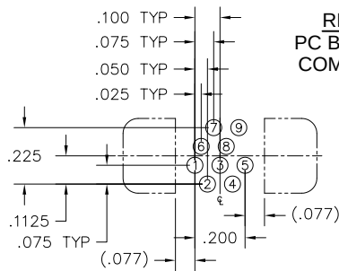
9 POSITION
