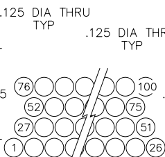
100 POSITION
