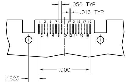
RECEPTACLE PC BOARD LAYOUT CIRCUIT SIDE
