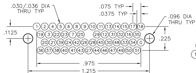
PLUG PC BOARD LAYOUT COMPONENT SIDE
