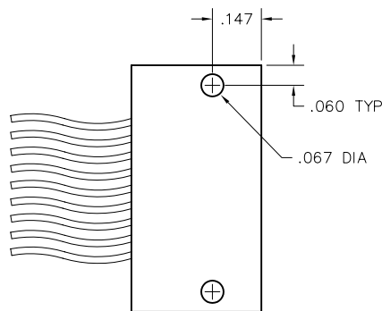
PLUG
