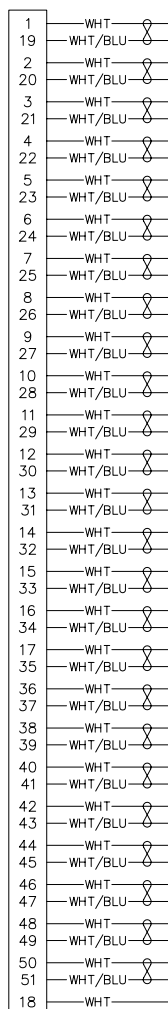
51 POSITION 3 rows
