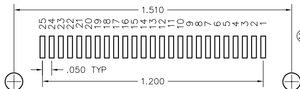
25 POSITION
