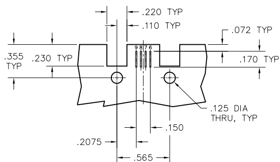
RECEPTACLE PC BOARD LAYOUT COMPONENT SIDE
