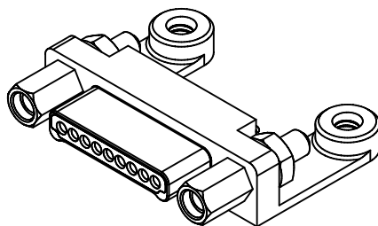
MK-172-009-175-220S (PLUG)
