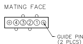
RECEPTACLE MA-1J1-004-245-A6700
