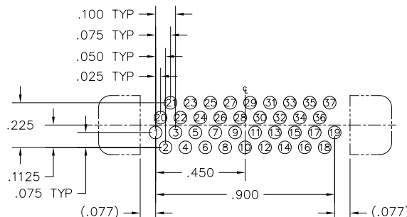
37 POSITION
