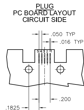
PC BOARD LAYOUT CIRCUIT SIDE
