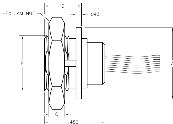
RECEPTACLE REAR PANEL MOUNT (Pin Contacts)
