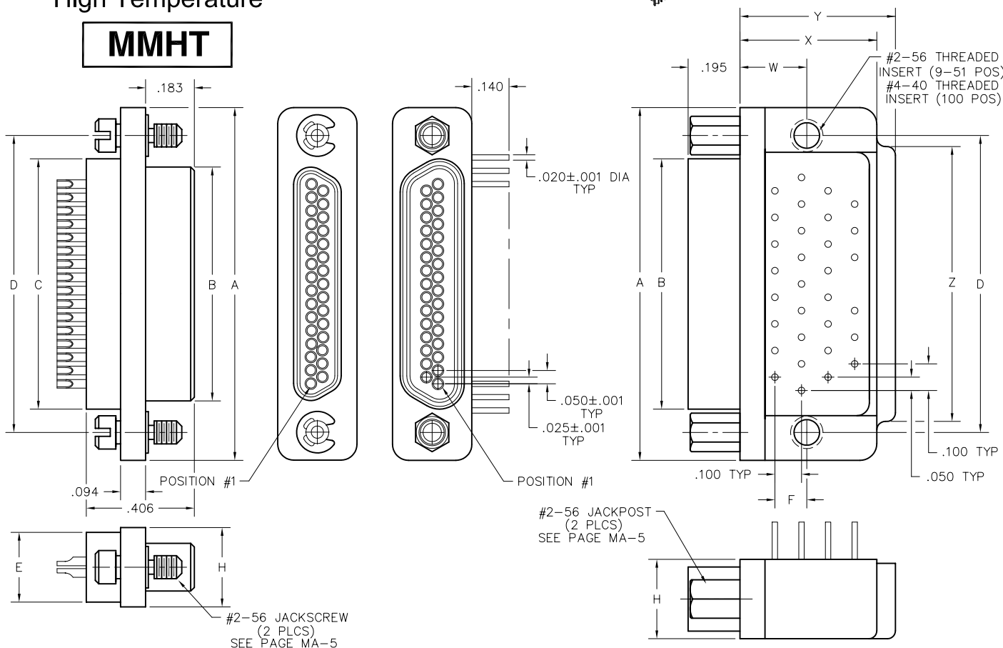
PLUG
