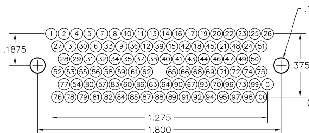
100 POSITION
