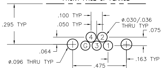
FRONT FACE OF FLANGE
