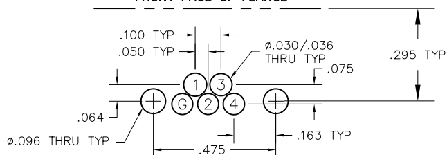
FRONT FACE OF FLANGE
