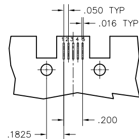
RECEPTACLE PC BOARD LAYOUT CIRCUIT SIDE
