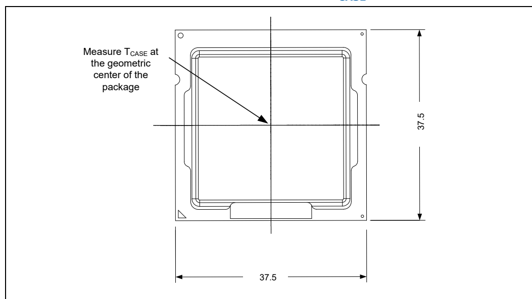
Figure 5-2. Thermal Test Vehicle (TTV) Case Temperature ( T_{\text{CASE}} ) Measurement Location
