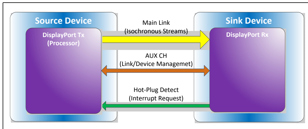
Figure 2-8. DisplayPort Overview
