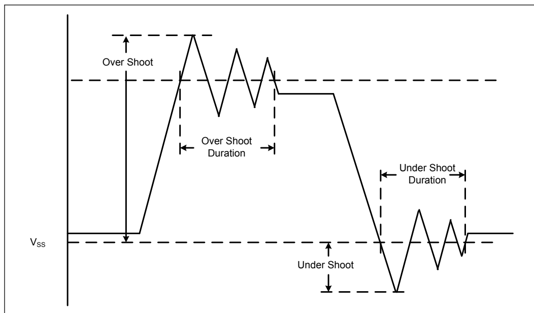
Figure 11. Maximum Acceptable Overshoot/Undershoot Waveform
