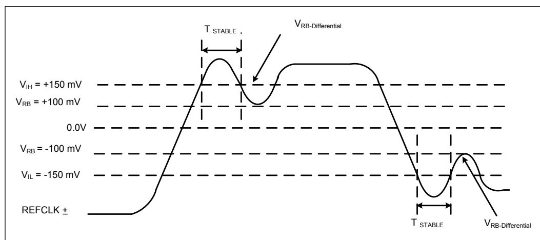
Figure 6. BCLK{0/1} Differential Clock Measurement Point for Ringback
