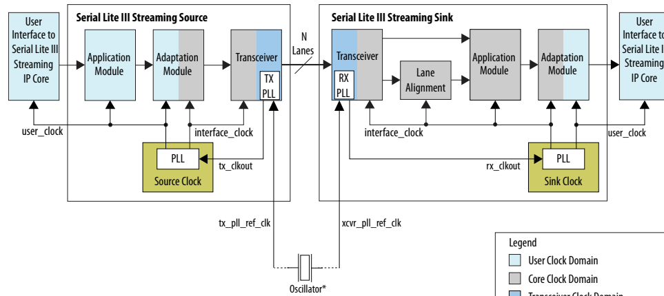
Figure 19. Standard Clocking Mode Structure for Stratix V or Arria V Devices
