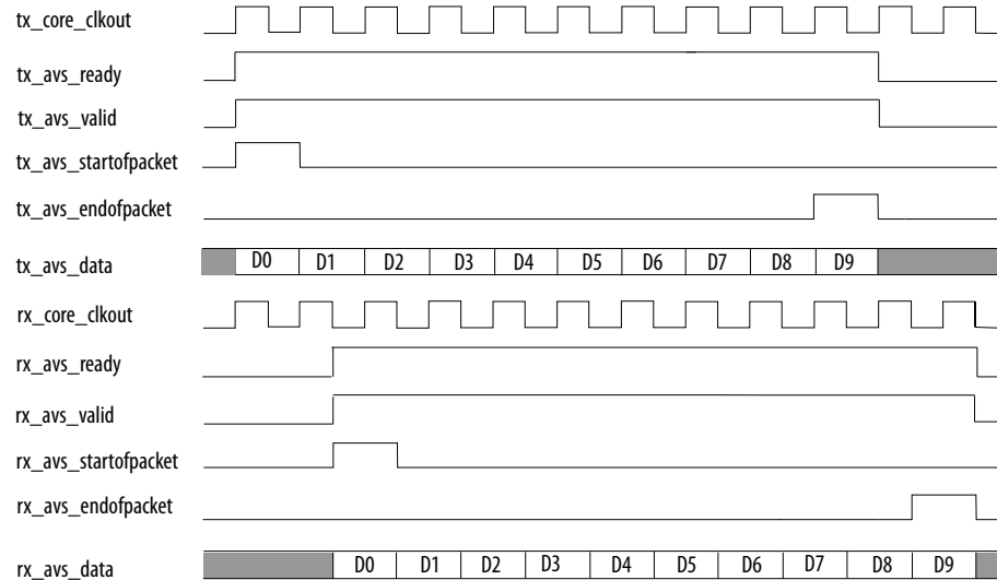
Figure 3. Full Mode Data Transfer
