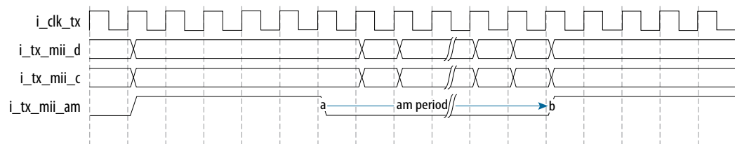
Figure 43. Inserting Alignment Markers
