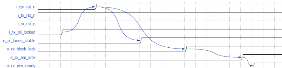
Figure 35. TX Datapath Reset Sequence
