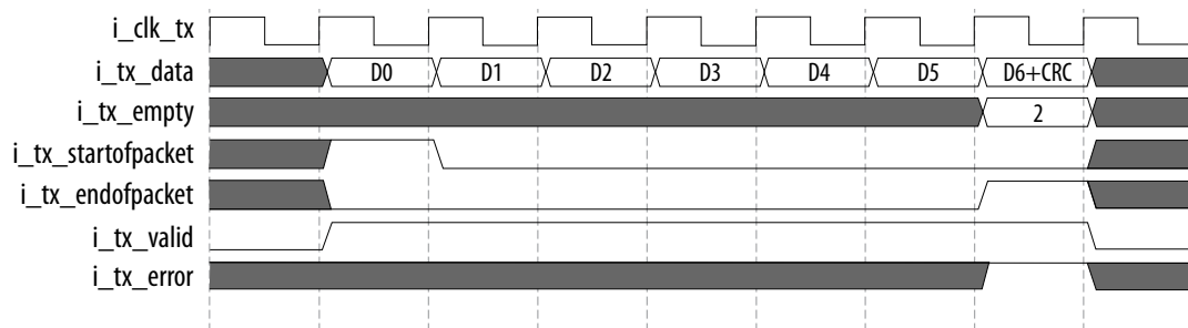
Figure 39. Using i_tx_error
