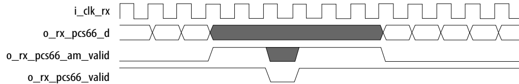
Figure 50. Receiving Alignment Markers for OTN Mode
