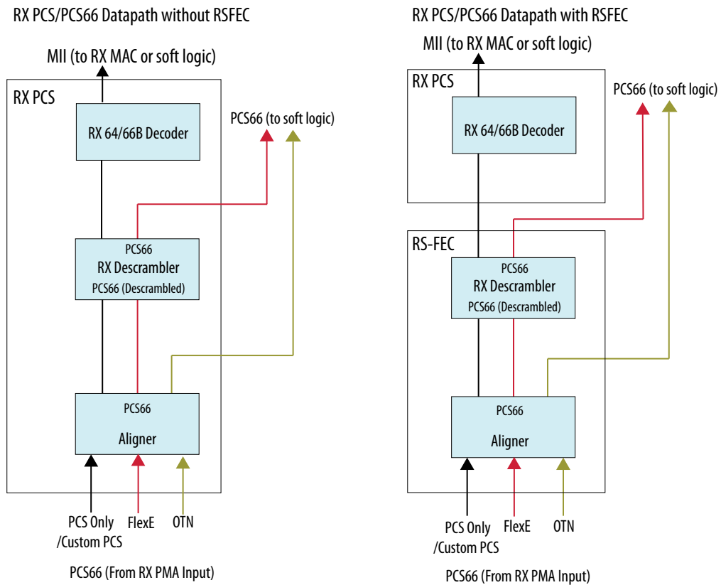
Figure 31. RX PCS Datapath with and without RS-FEC
