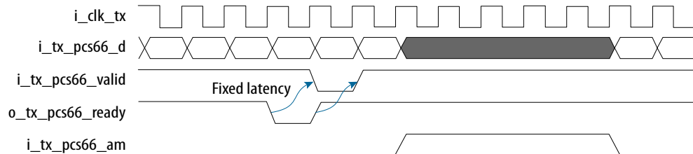
Figure 46. Transmitting Data Using the PCS66 TX Interface
