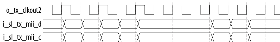
Figure 89. Transmitting Data Using TX MII Interface
