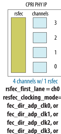
Figure 81. Four 24.33024 Gbps Channels with RS-FEC
