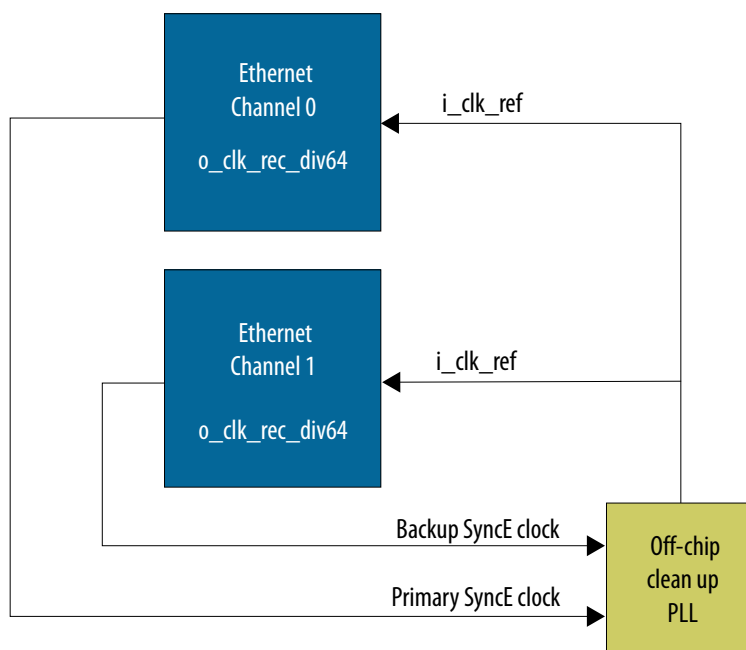
Figure 55. Clock Connection in SyncE Operation
