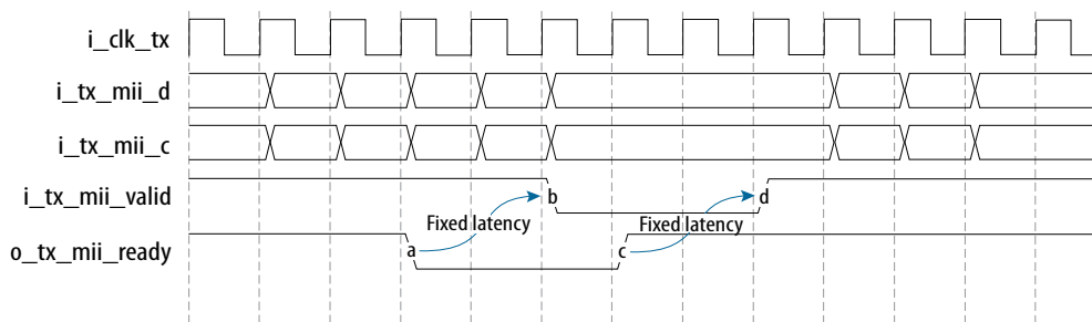
Figure 51. Transmitting Data Using the PCS Mode TX Interface
