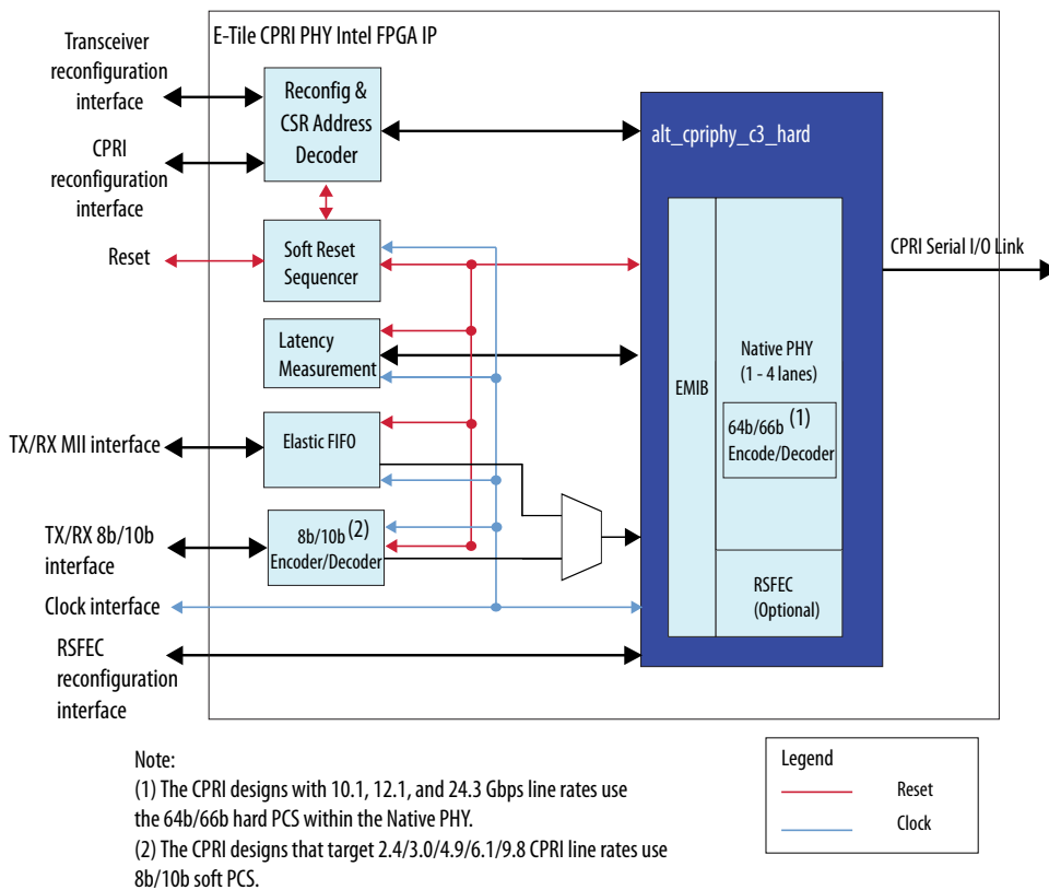
Figure 72. E-Tile CPRI PHY IP Block Diagram
