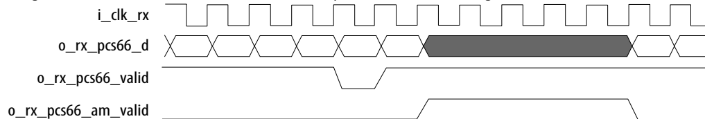
Figure 48. Receiving Data Using the PCS66 RX Interface
