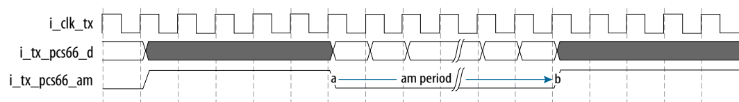
Figure 47. Inserting Alignment Markers
