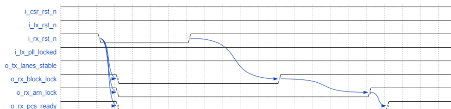
Figure 36. RX Datapath Reset Sequence
