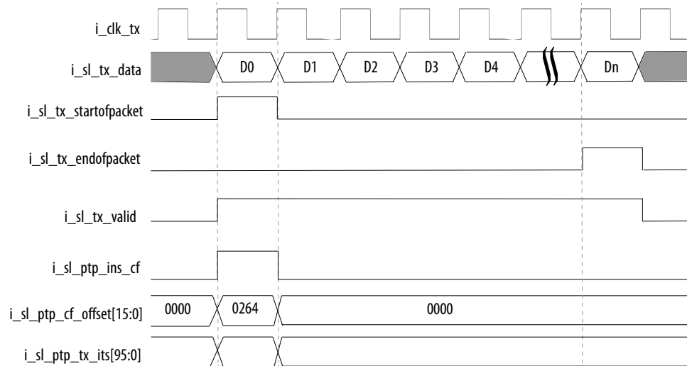
Figure 26. Example Waveform for 1-step TX Timestamp using i_sl_ptp_ins_cf Signal
