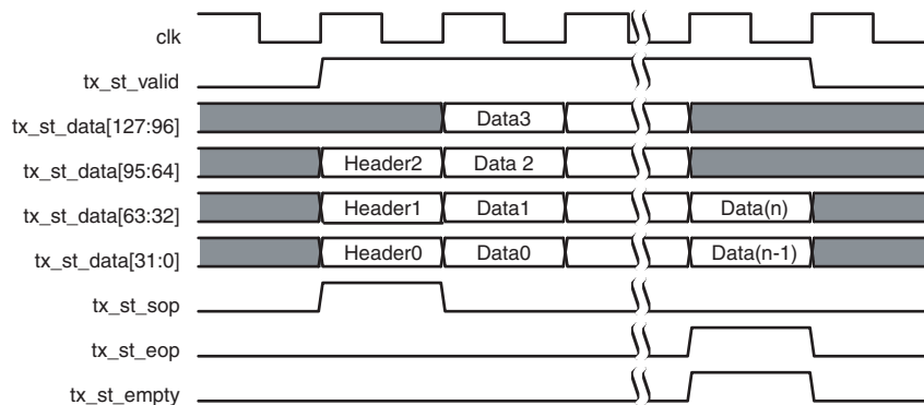
Figure 5-20. 128-Bit Avalon-ST tx_st_data Cycle Definition for 3-DWord Header TLP with QWord Aligned Address
