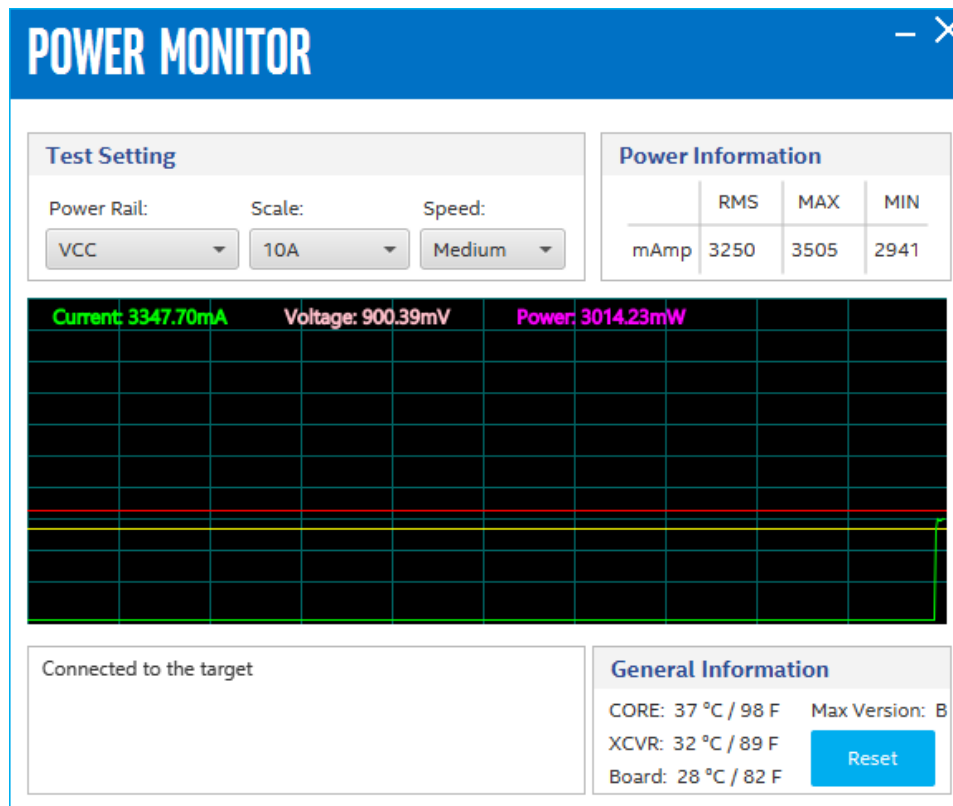
Figure 43. Power Monitor
