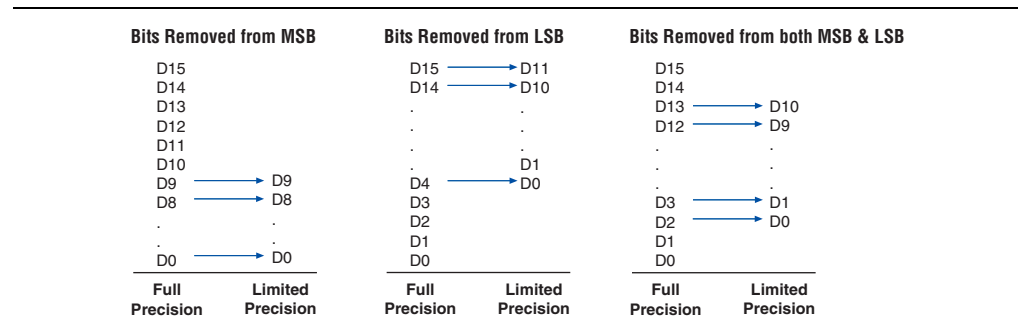
Figure 3–1. Removing Bits from the MSB and LSB
