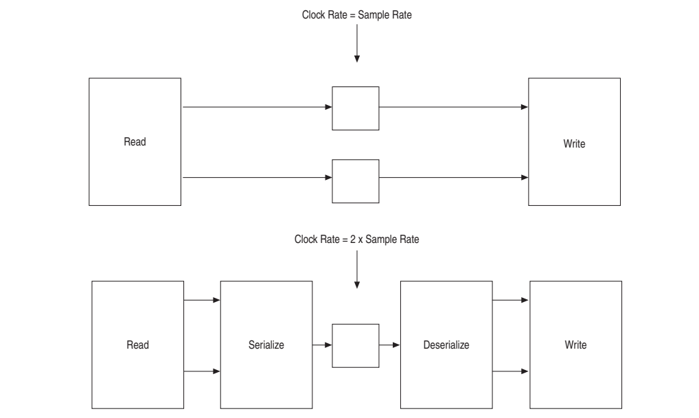
Figure 4-8. Time-Division Multiplexing to Save Hardware Resources
