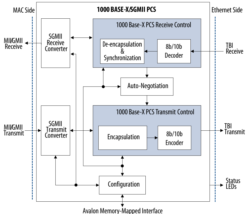
Figure 25. 1000BASE-X/SGMII PCS
