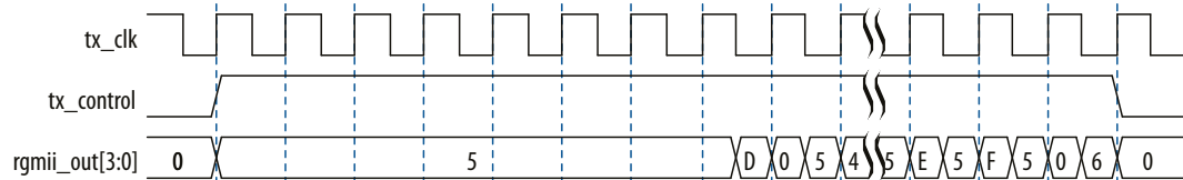
Figure 70. RGMII Transmit in Gigabit Mode
