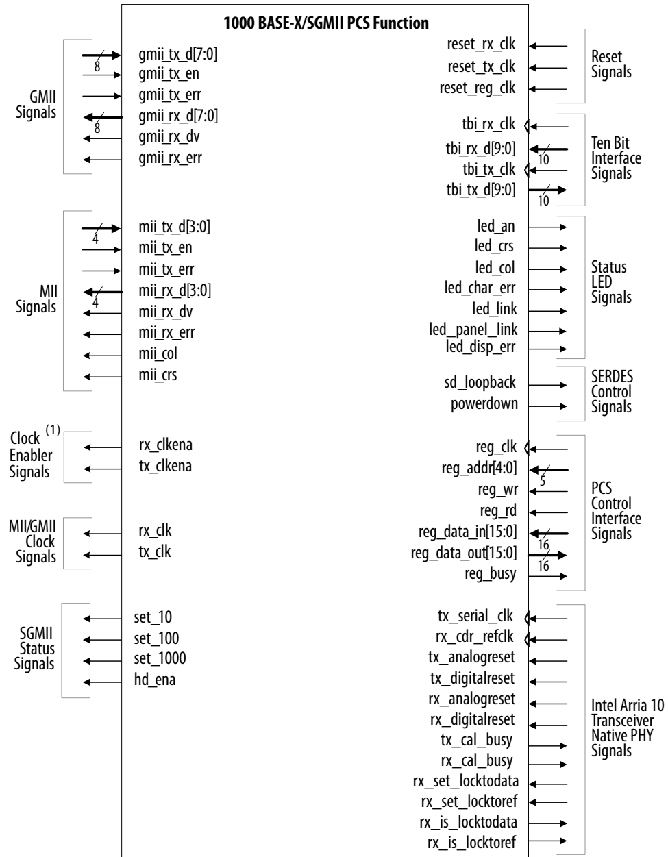
Figure 59. 1000BASE-X/SGMII PCS Function Signals
