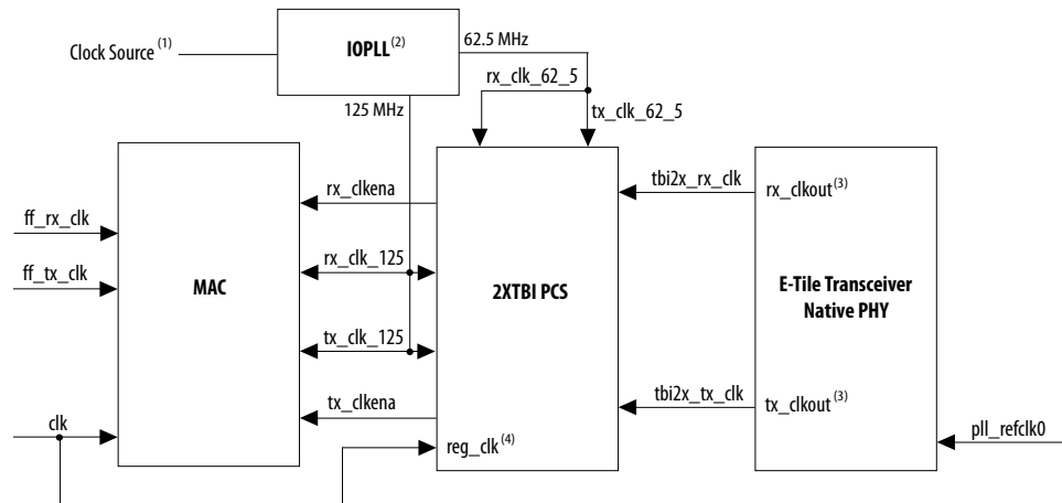
Figure 83. Clock Connectivity in MAC with 2XTBI PCS and Embedded PMA
