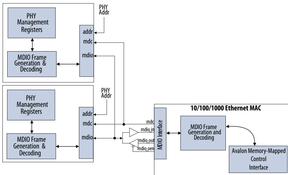
Figure 20. MDIO Interface
