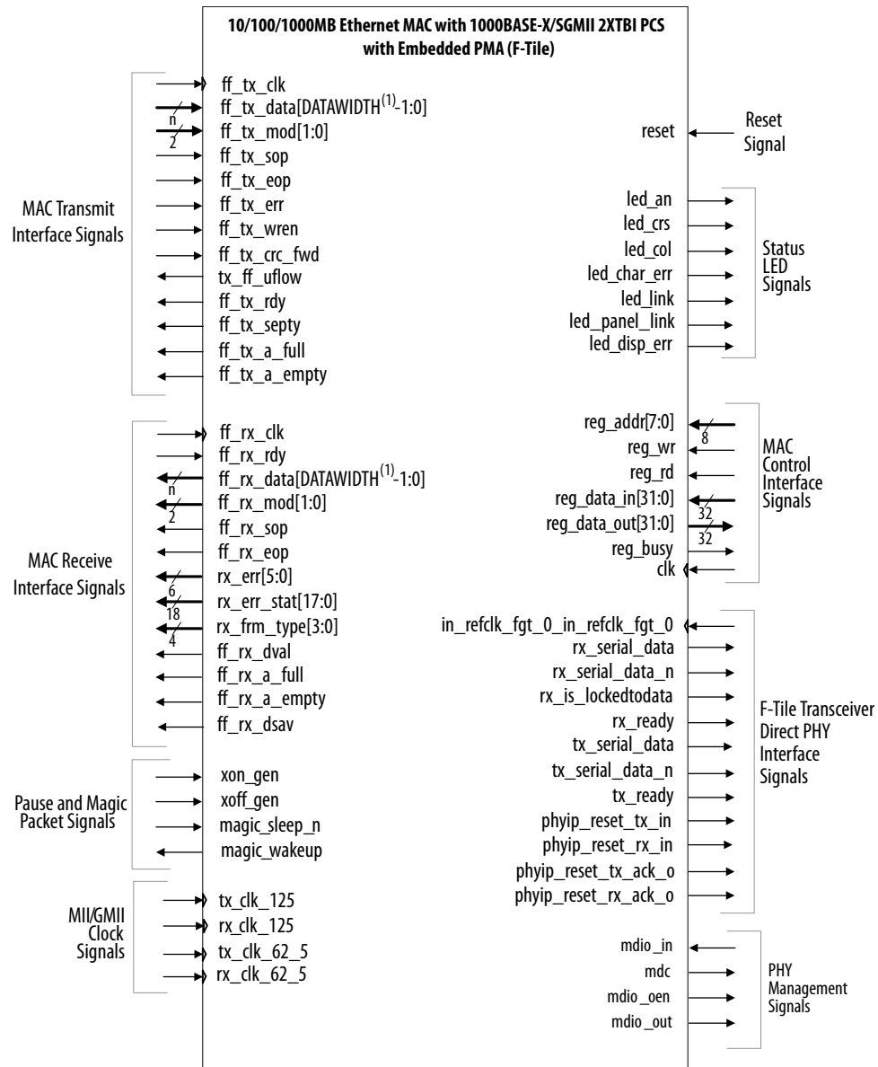
Figure 52. 10/100/1000 Ethernet MAC Function with Internal FIFO Buffers, and 1000BASE-X/SGMII 2XTBI PCS Signals With Embedded PMA Signals (F-Tile)
