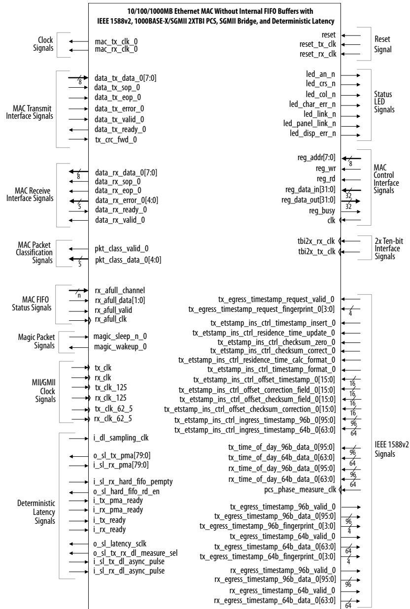
Figure 55. 10/100/1000 Ethernet MAC Function Without Internal FIFO Buffers with IEEE 1588v2, 1000BASE-X/SGMII 2XTBI PCS, SGMII Bridge, and Deterministic Latency Signals
