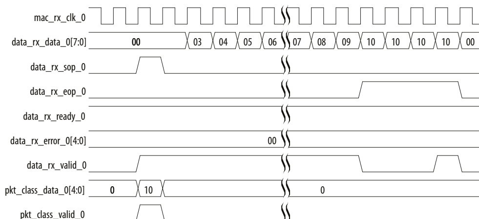
Figure 64. Receive Operation—MAC Without Internal FIFO Buffers
