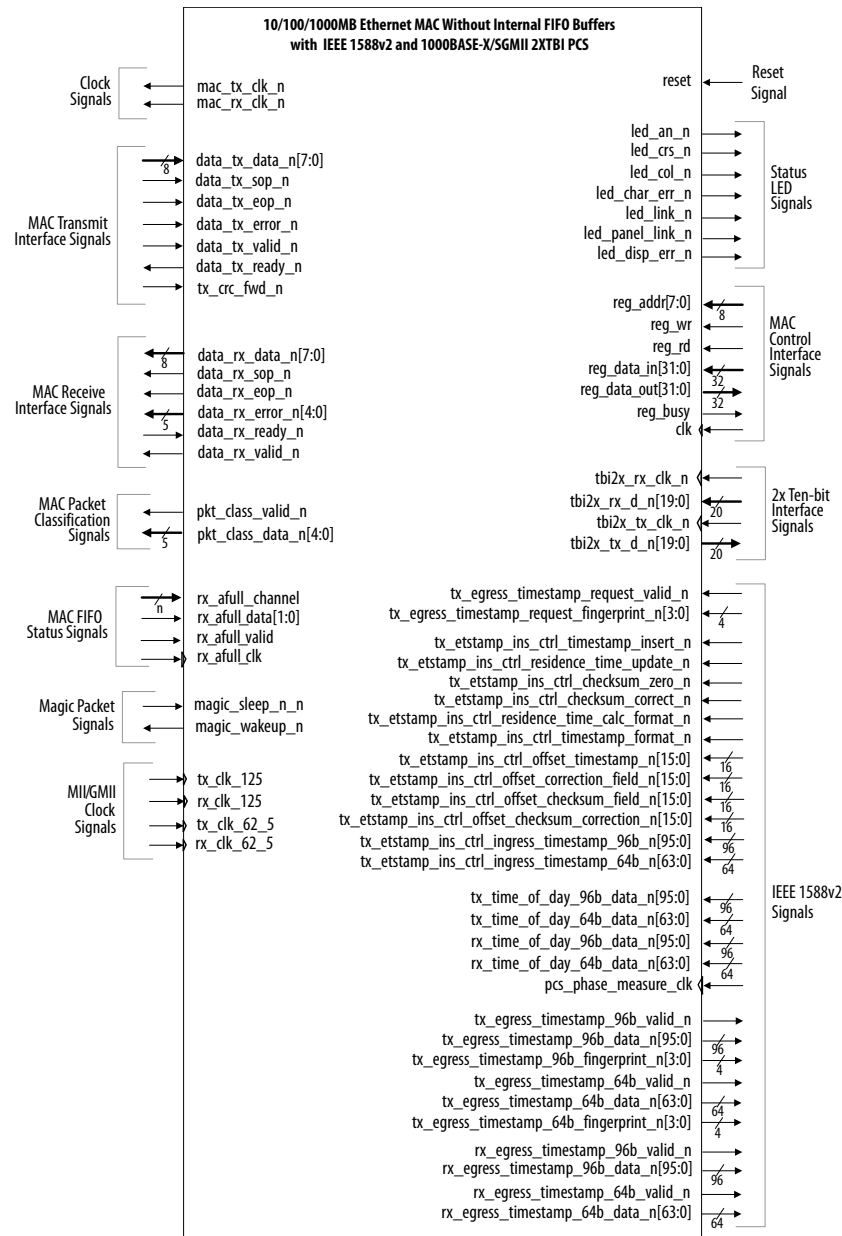
Figure 54. 10/100/1000 Ethernet MAC Function Without Internal FIFO Buffers with IEEE 1588v2 and 1000BASE-X/SGMII 2XTBI PCS Signals
