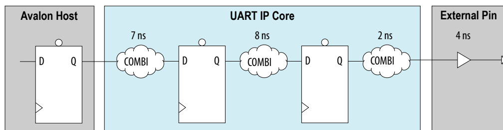
Figure 34. Maximum Delays on UART
