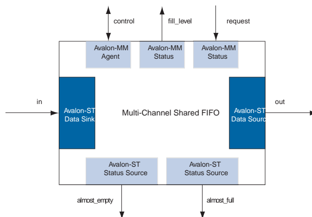
Figure 2. Avalon-ST Multi-Channel Shared Memory FIFO Core
