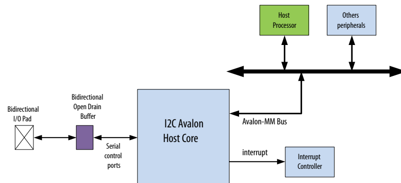
Figure 45. Intel FPGA Avalon I 2 C Host Core without DMA
