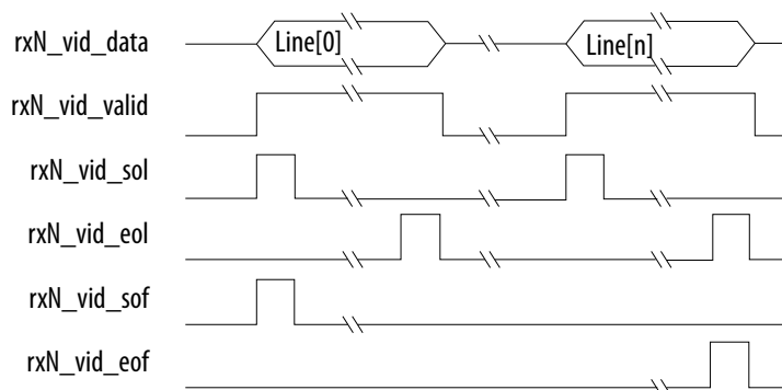
Figure 29. Video Out Image Port Timing Diagram
