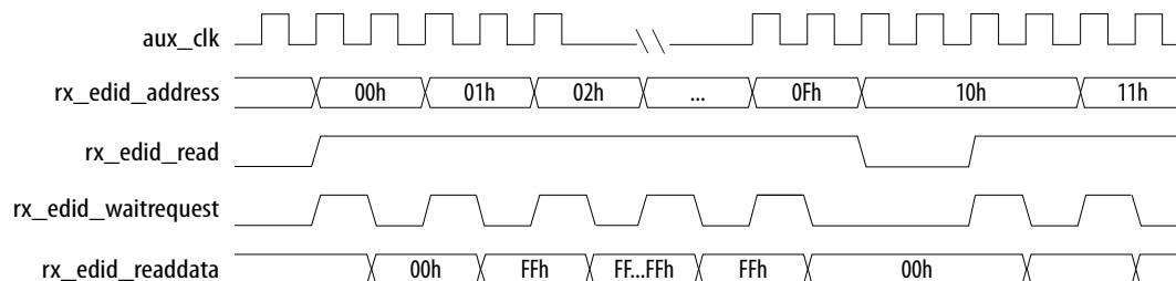
Figure 35. rx_edid Interface
