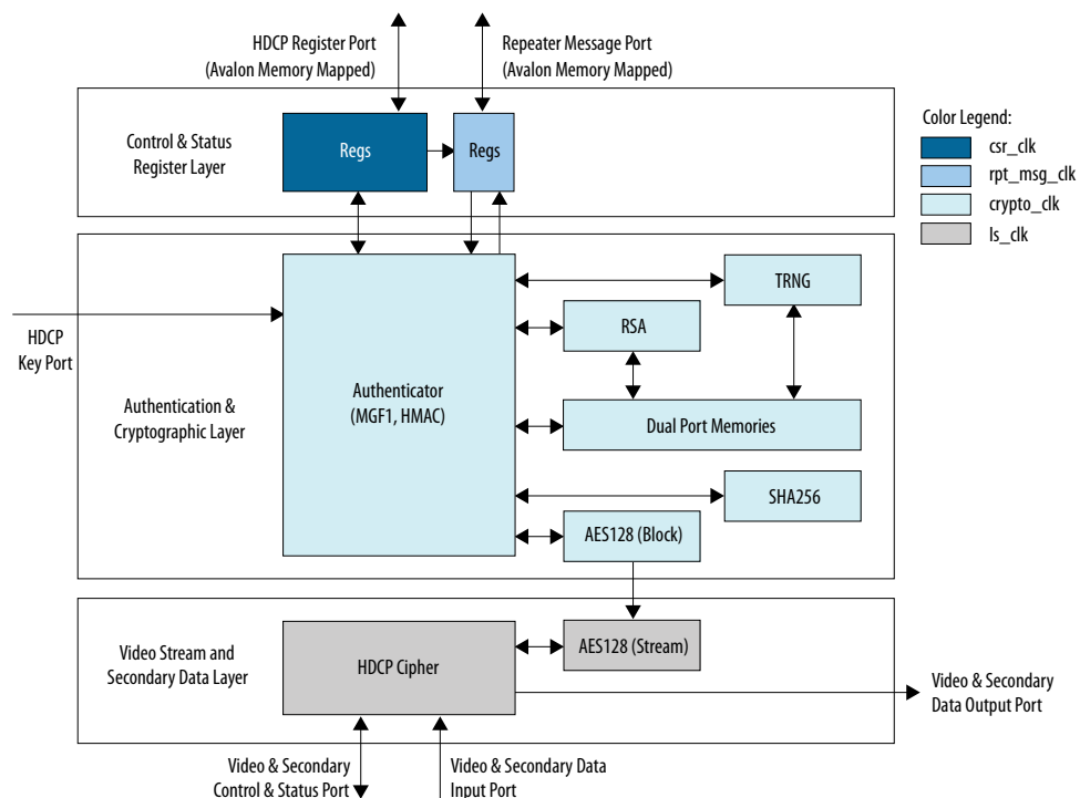
Figure 28. Architecture Block Diagram of HDCP 2.3 RX IP
