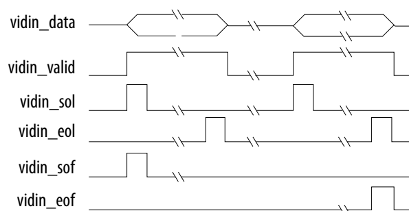
Figure 8. Video Input Port Timing Diagram
