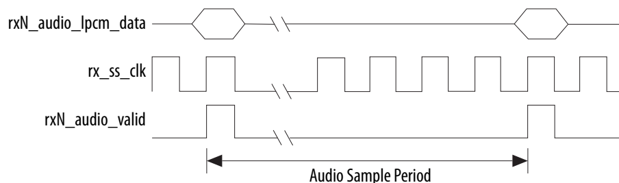
Figure 34. rxN_audio Data Output
