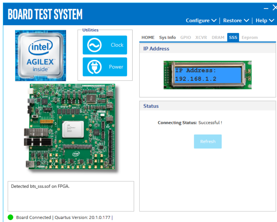
Figure 15. The SSS Tab
