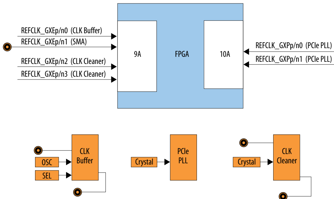
Figure 20. Transceiver Clocks
