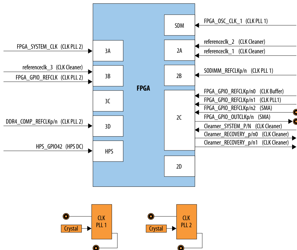
Figure 20. Transceiver Clocks
