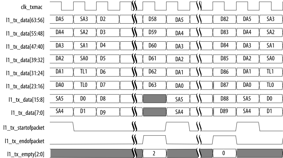
Figure 25. Octet Transmission on the 25GbE Avalon Streaming Signals
