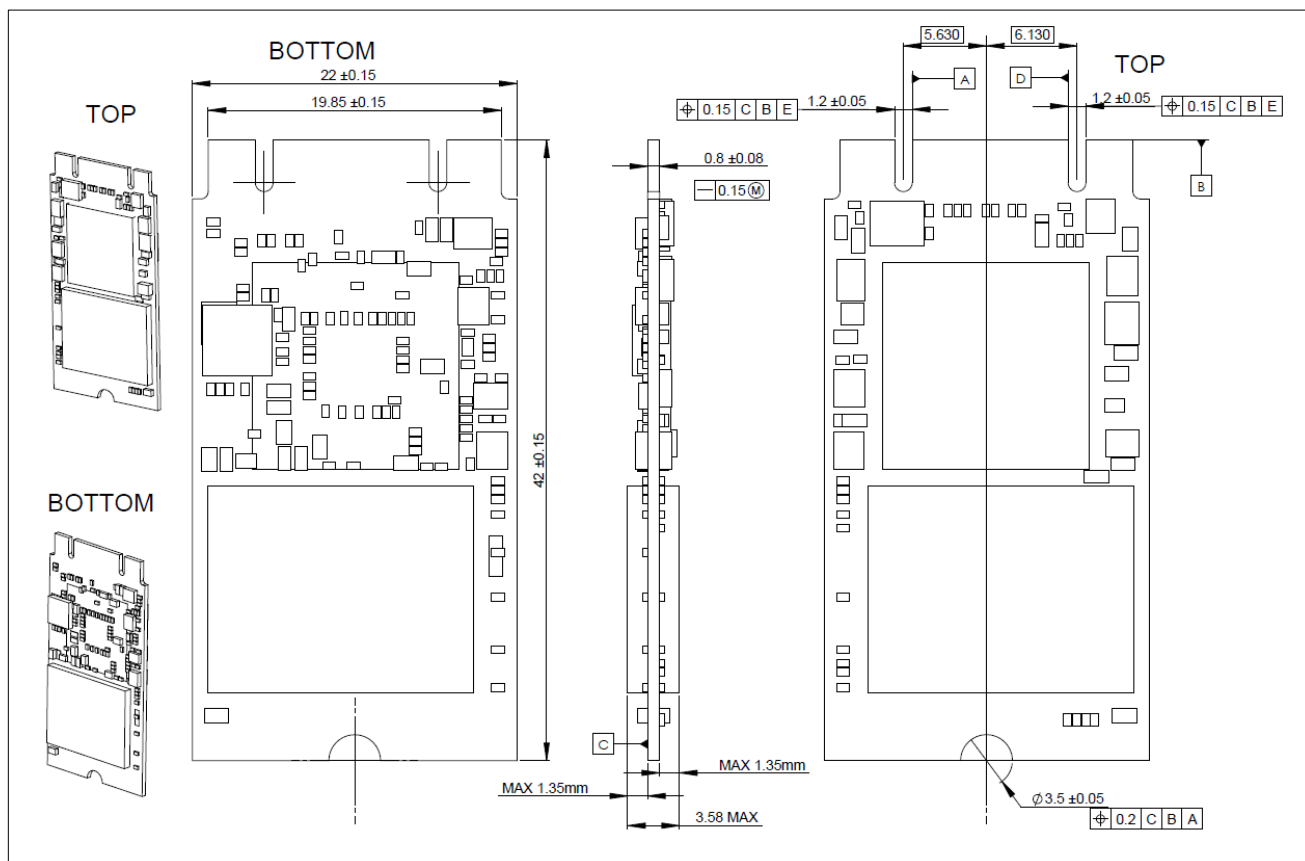
Figure 3: Dimensions for 42 mm Double-Sided M.2 Form Factor (2242-D2-B-M) 120 GB
