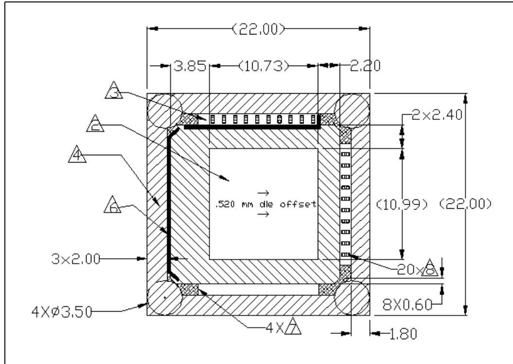
Figure 7. Package Dimensions (Top View)
