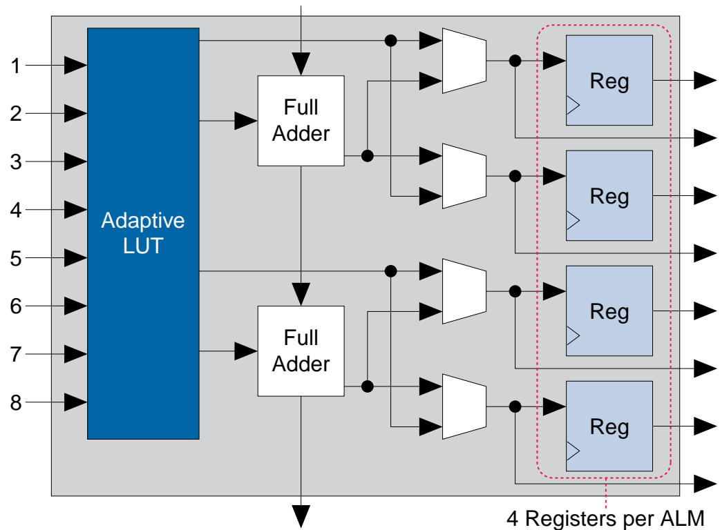
Figure 11. Stratix 10 FPGA and SoC ALM Block Diagram
