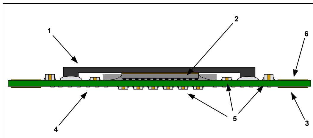
Figure 4-1. Processor Package Assembly Sketch
