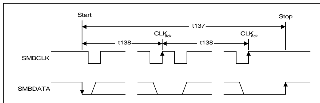
Figure 22-17. SMBus Timeout
