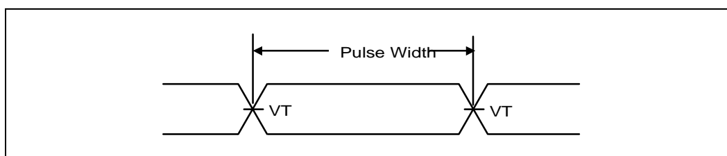
Figure 22-5. Pulse Width
