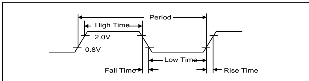
Figure 22-1. Clock Timing
