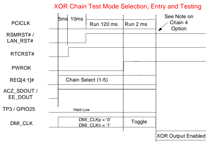
Figure 24-1. XOR Chain Test Mode Selection, Entry and Testing
