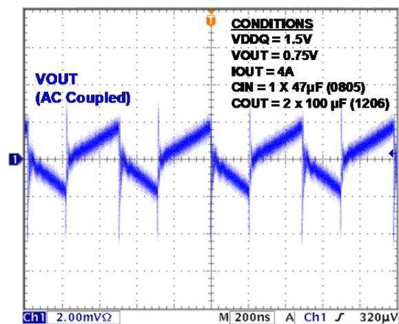
Output Ripple at Full Bandwidth
