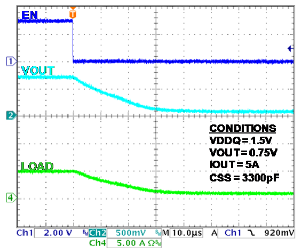
Shutdown with Enable
