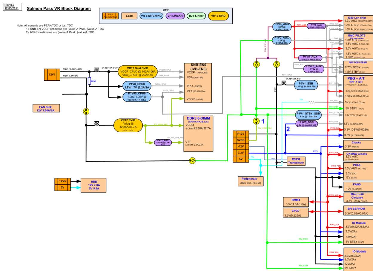
Figure 31. Power Distribution Block Diagram
