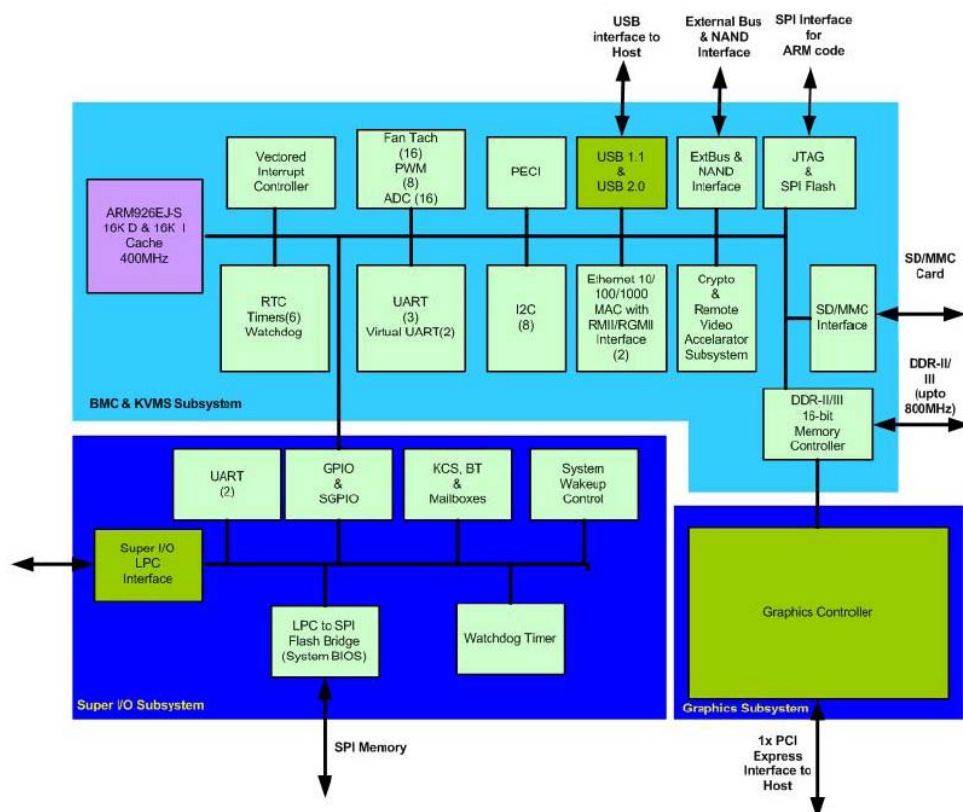
Figure 23. Integrated BMC Hardware
