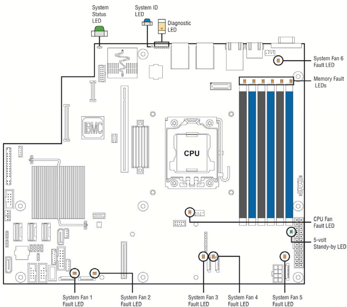
Figure 29. On-Board Diagnostic LED Placement
