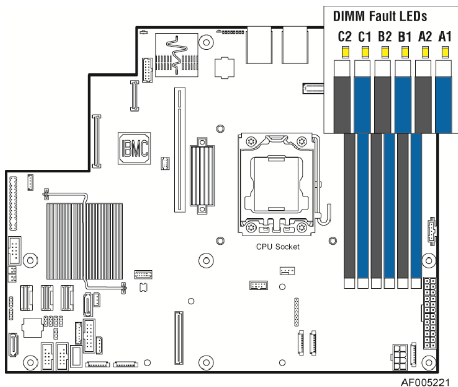
Figure 30. Memory Slot Fault LED Locations
