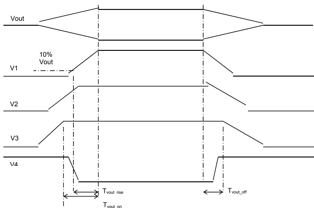
Figure 32. Output Voltage Timing
