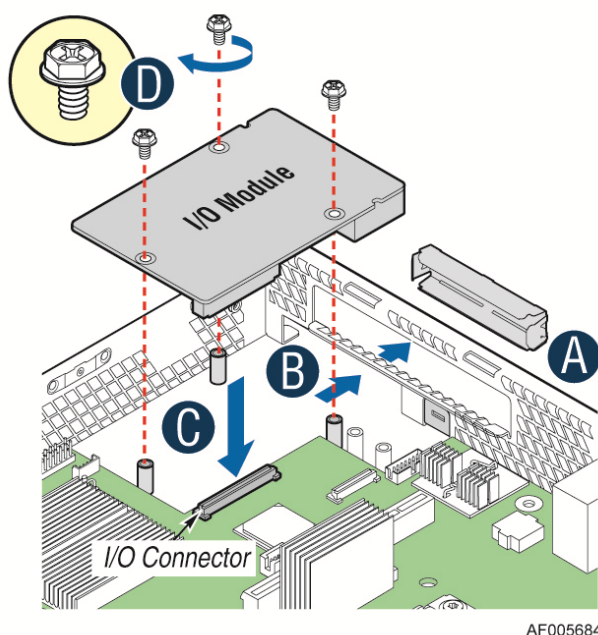
Figure 19. Server Board Layout - I/O Module Connector
