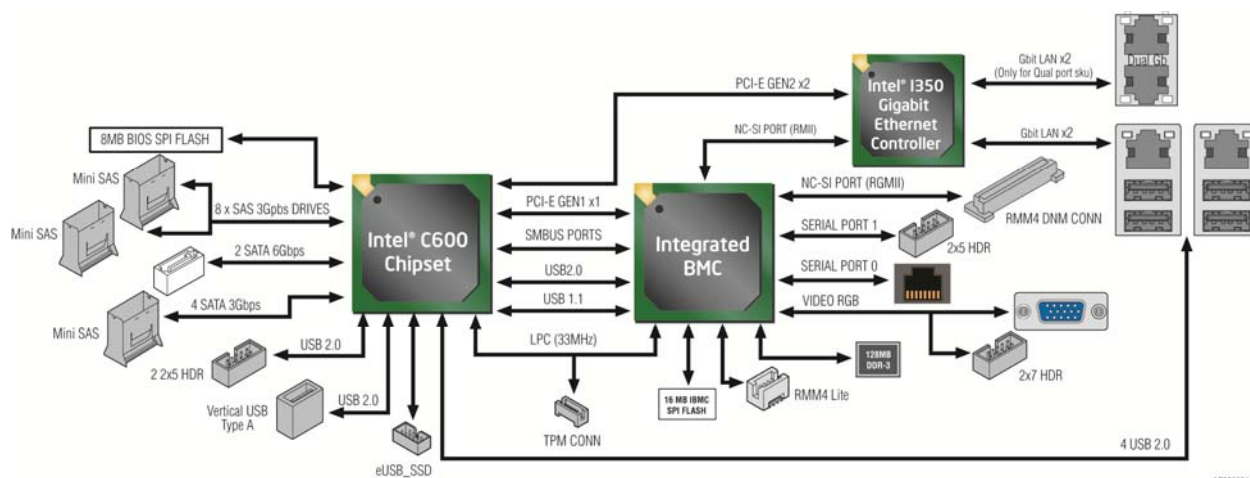
Figure 20. Functional Block Diagram – Chipset Supported Features and Functions
