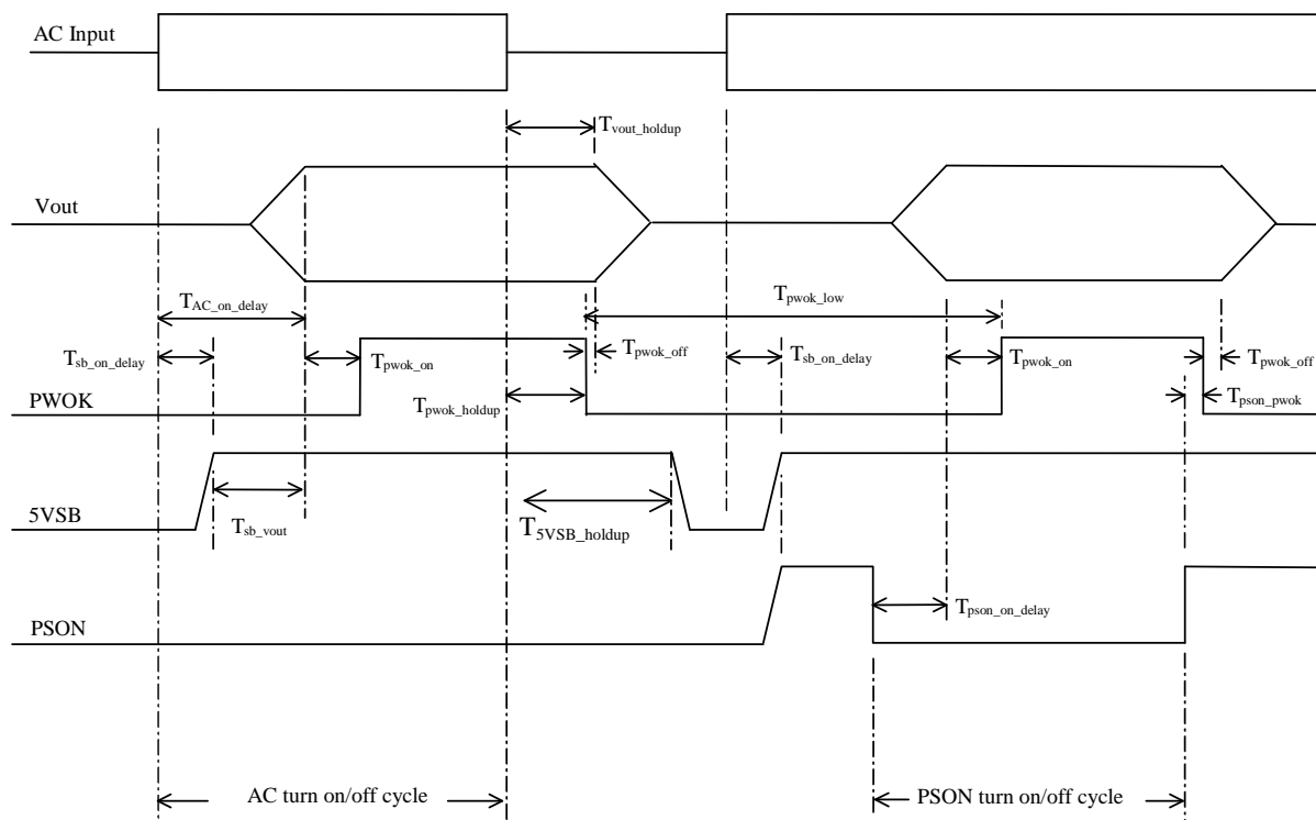
Figure 33. Turn On/Off Timing (Power Supply Signals)
