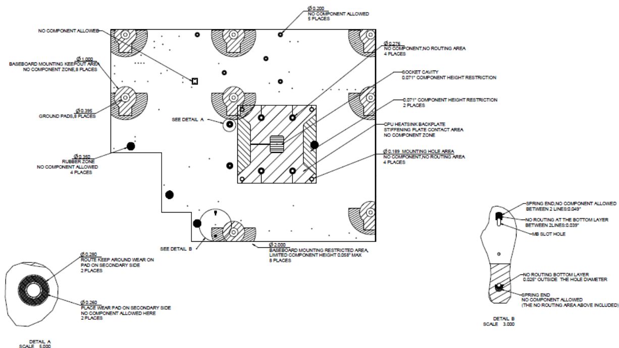
Figure 11. Intel® Server Boards S1400SP – Second Side Keepout Zone
