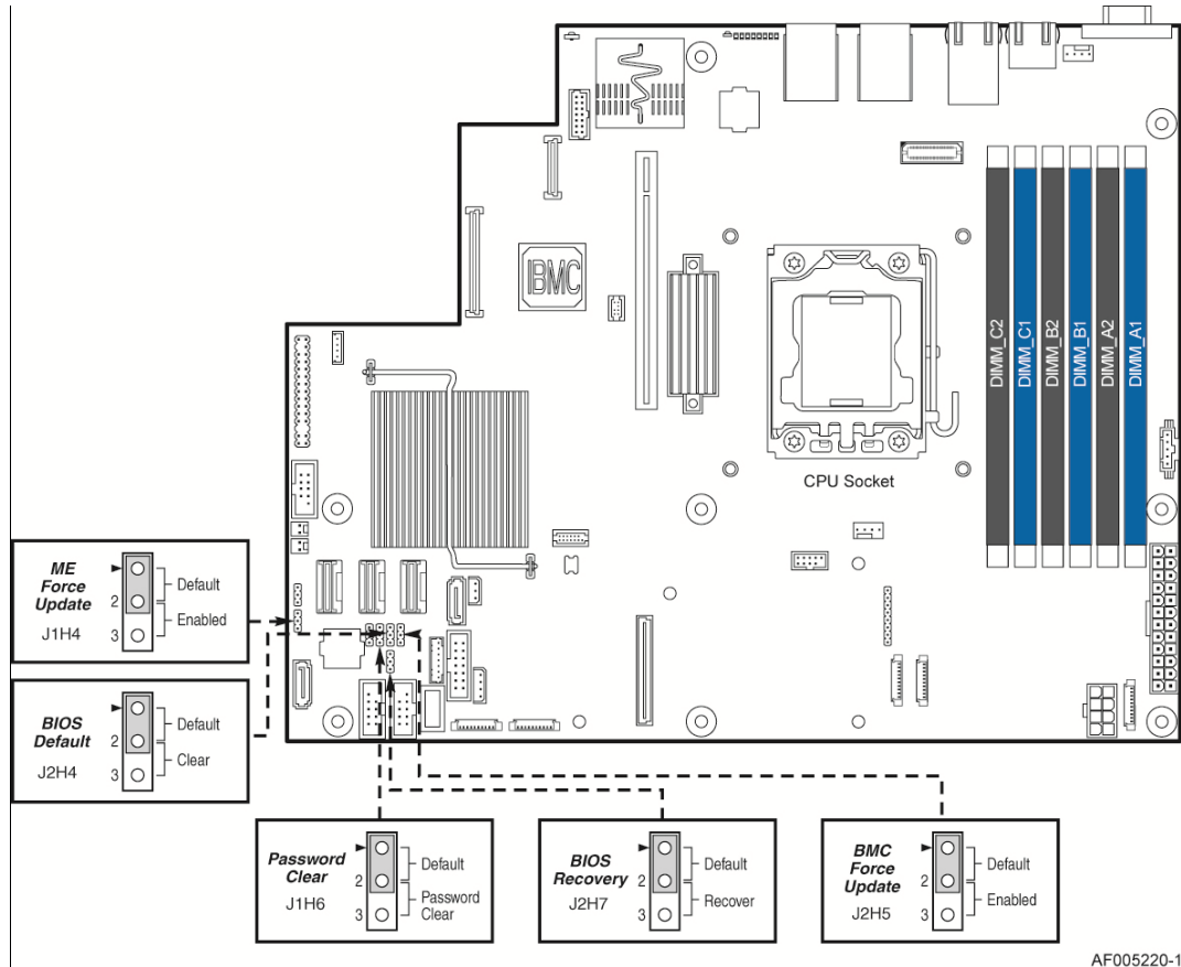
Figure 28. Jumper Blocks
