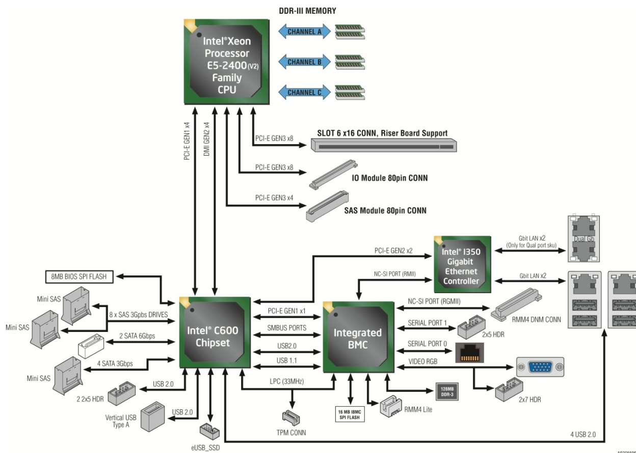
Figure 14. Intel® Server Board S1400SP Functional Block Diagram
