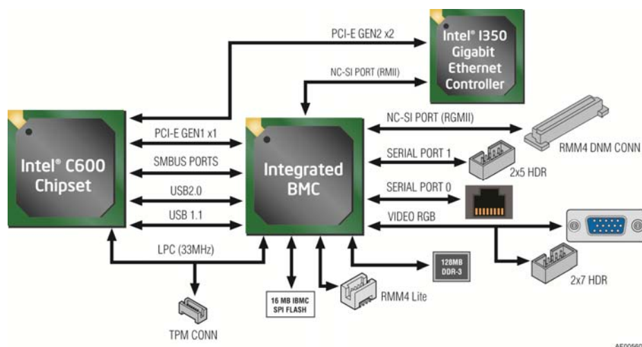
Figure 22. Integrated Baseboard Management Controller (BMC) Overview
