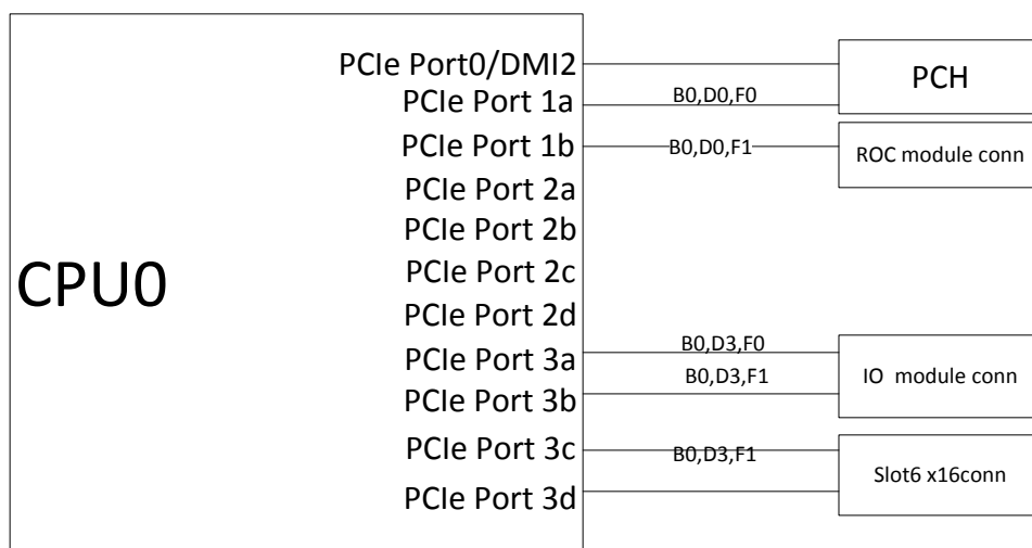
Figure 18. PCI Express* Lane Mapping
