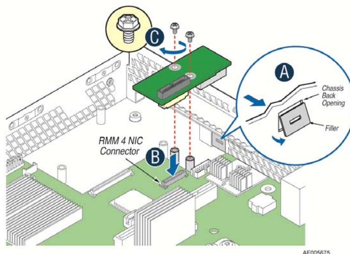
Figure 27. Intel® RMM4 Dedicated Management NIC Installation
