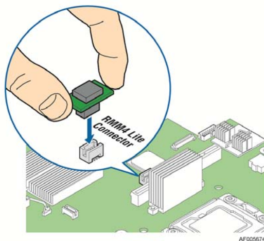
Figure 26. Intel® RMM4 Lite Activation Key Installation
