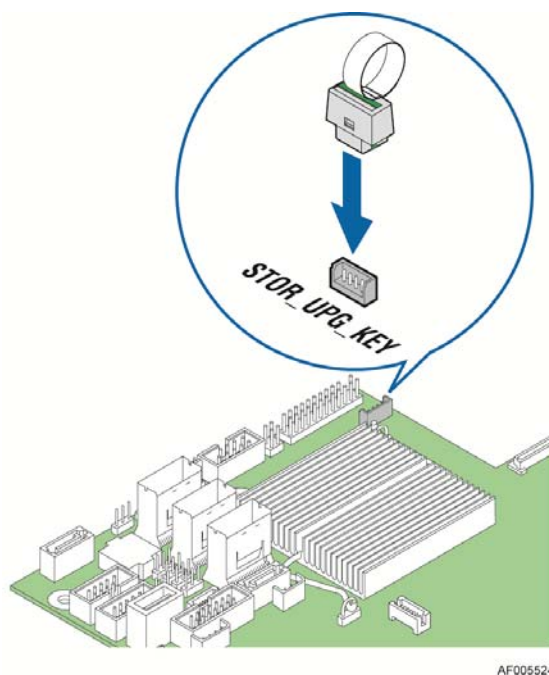
Figure 21. Intel® RAID C600 Upgrade Key Connector
