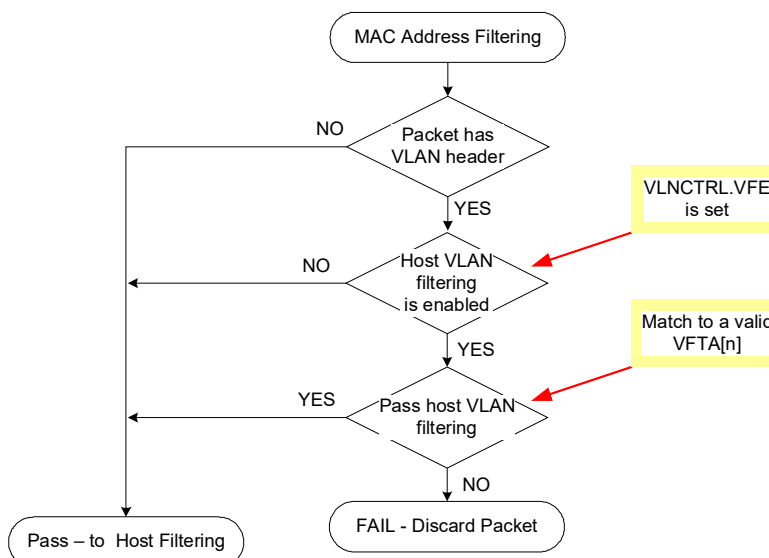
Figure 7-3. VLAN Filtering
