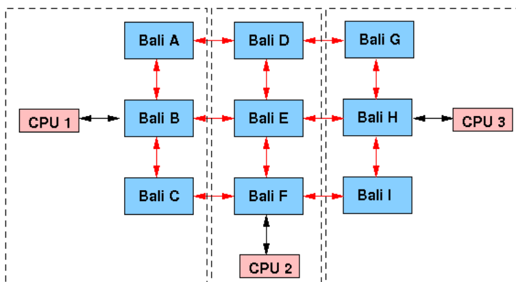
Figure 5-22 Multiple CPUs
