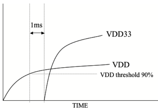
Figure 15-1 Power Supply Sequencing
