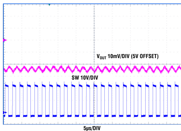
FIGURE 20. NON-SYNCHRONOUS BUCK, FORCE PWM MODE, V_{PVIN} 12V, 2A
