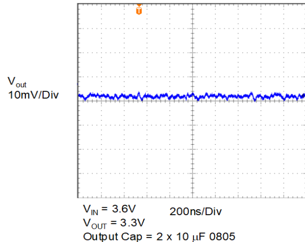
Output Ripple
