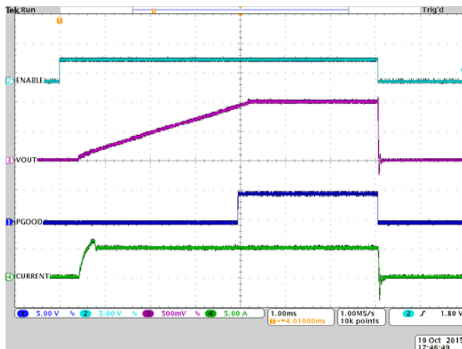
Figure 16: Startup V_{IN} = 5V , V_{OUT} = 1V , I_L = 6A
