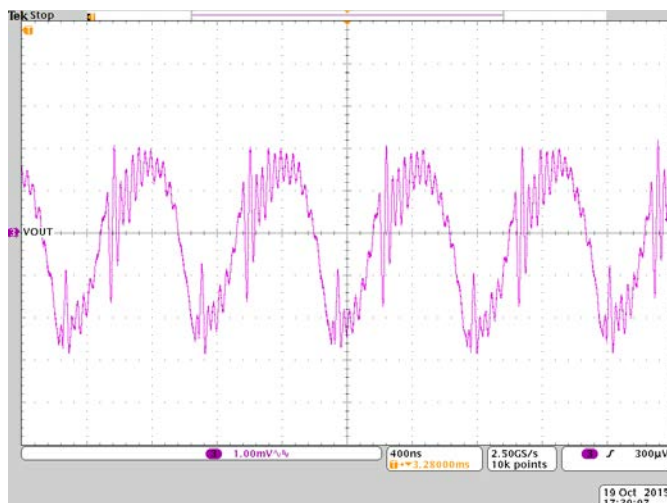
Figure 14: Output ripple V_{IN} = 5V , V_{OUT} = 1.8V
