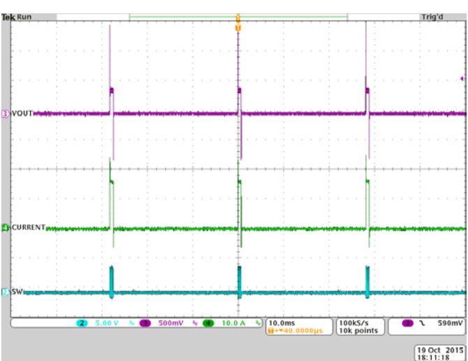
Figure 20: Hiccup mode during short-circuit protection
