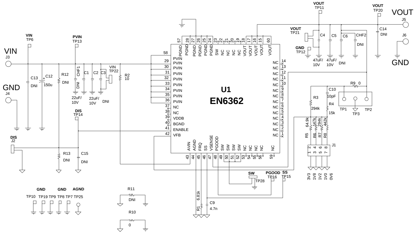
Figure 2: Evaluation Board Schematic
