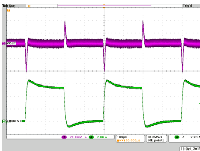
Figure 18: 0/6A load transient
