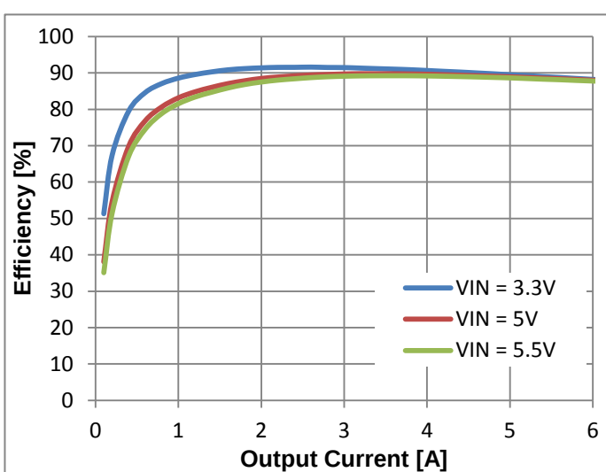
Figure 6: Efficiency – V_{OUT} = 1V
