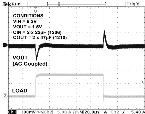
Load Transient from 0 to 8A
