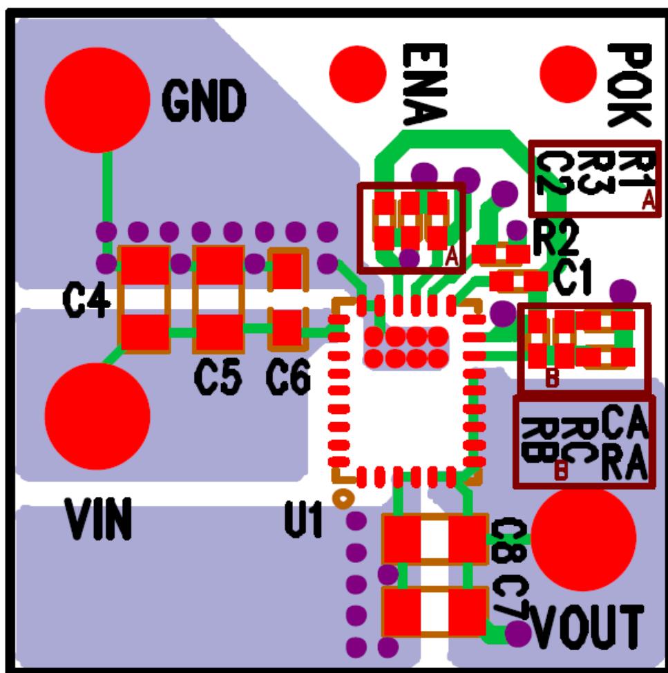
Recommendation 1: Input and output filter capacitors should be placed on the same side of the PCB, and as close to the EN6310QA package as possible. They should be connected to the device with very short and wide traces. Do not use thermal reliefs or spokes when connecting the capacitor pads to the respective nodes. The Voltage and GND traces between the capacitors and the EN6310QA should be as close to each other as possible so that the gap between the two nodes is minimized, even under the capacitors.
