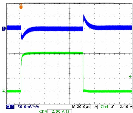
Transient Response 5.5V IN /1.2V OUT , 0-6A, 10A/μs. C_{OUT} = 50\mu F
