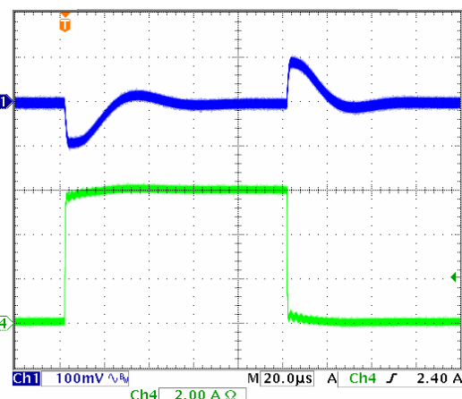
Transient Response 5.5V IN /3.3V OUT , 0-6A, 10A/μs. C_{OUT} = 50\mu F
