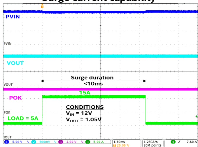
Surge current capability
