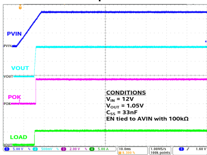
VIN Startup at 5A Load
