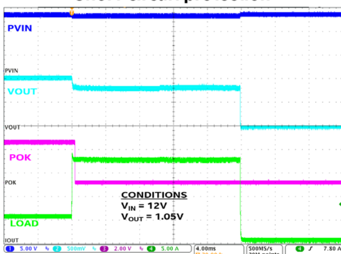
Short-circuit protection
