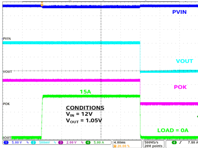
OCP during steady-state operation
