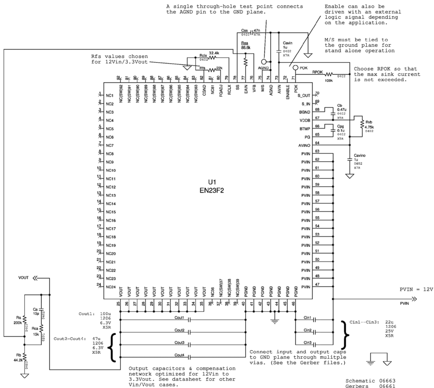
Figure 13: Engineering Schematic
