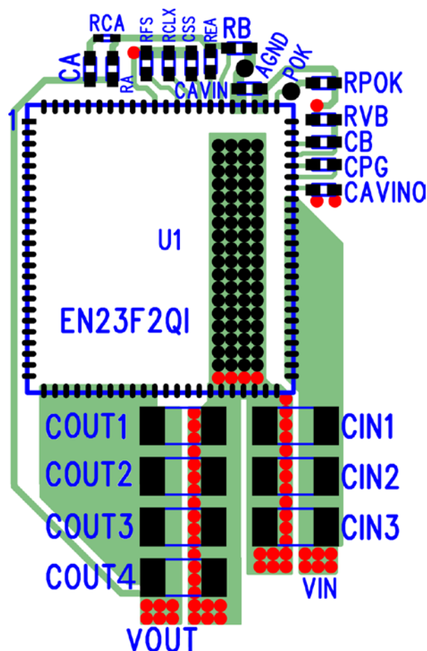
Figure 14: Top Layer Layout with Critical Components (Top View). See Figure 13 for corresponding schematic.
