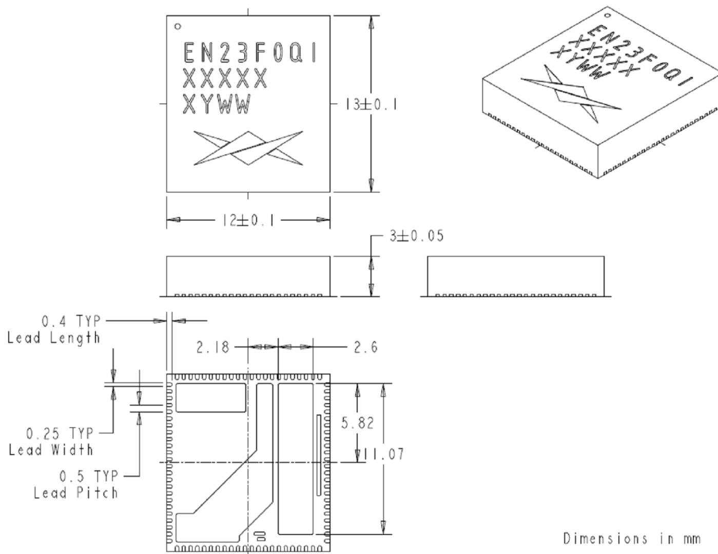
Figure 18: EN23F0QI Package Dimensions (Bottom View)
