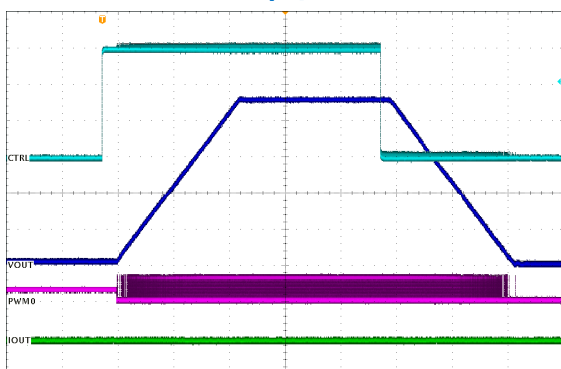
Start-up/Shutdown, CTRL at No Load, 800μs/div
