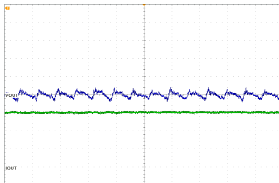
Output Voltage Ripple, 60A Load
