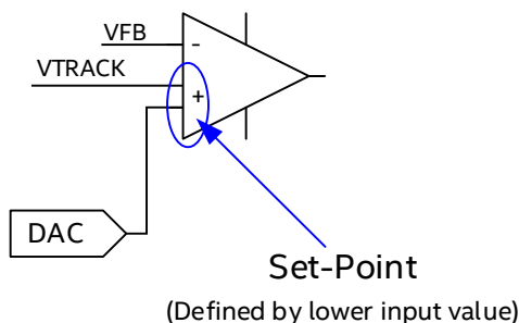
Figure 9: VTRACK Circuitry
