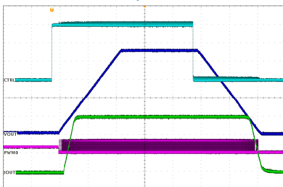
Start-up/Shutdown, CTRL At 60A Load, 800μs/div
