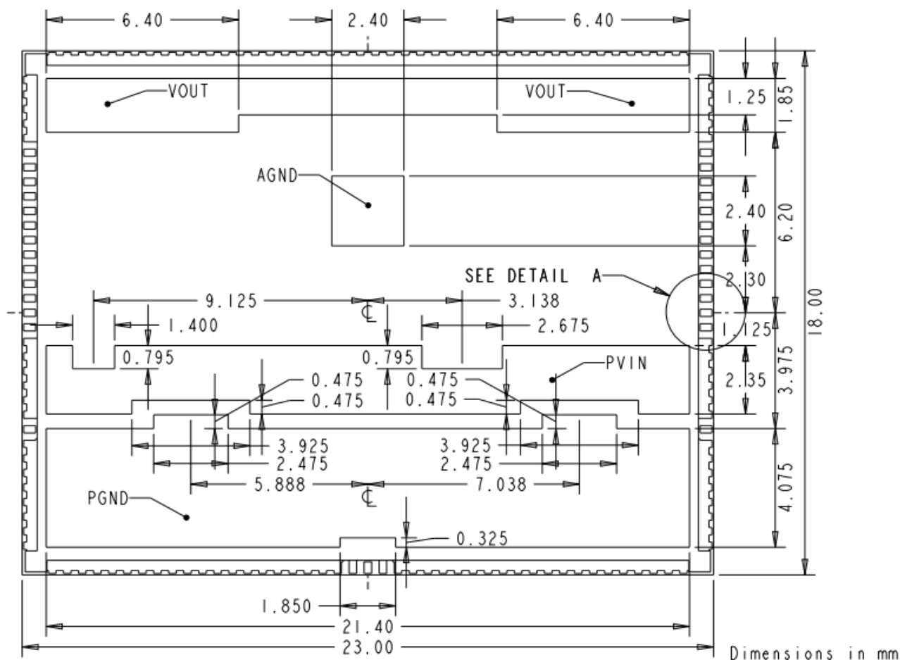
Figure 26: Package Dimensions 2/3
