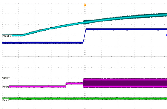
Start-up into 0.6V Pre-Bias With PVIN, 4ms/div
