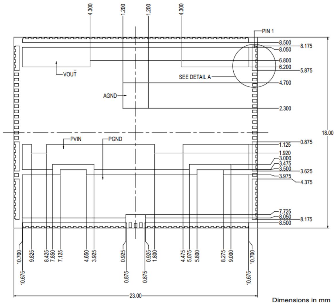
Figure 20: Package Bottom side (Bottom View)
