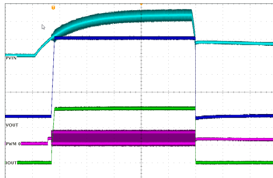
Start-up/Shutdown, PVIN at 60A Load, 20ms/div
