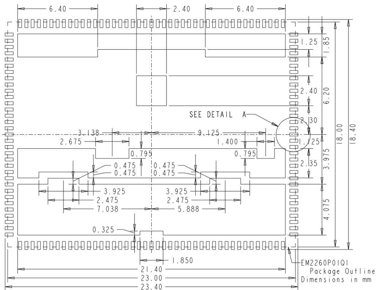
Figure 22: Recommended PCB Footprint (Top View)
