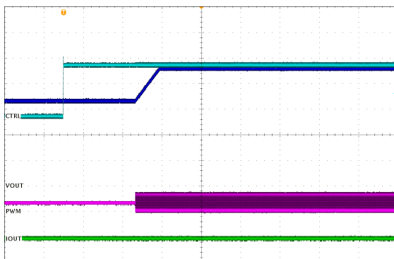
Start-up into 0.7V Pre-Bias With CTRL, 800μs/div
