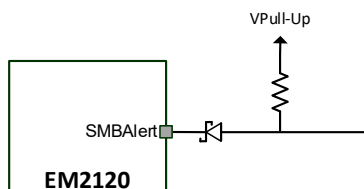
Figure 7: SMBAlert Pin Low Voltage Pull-up Option
