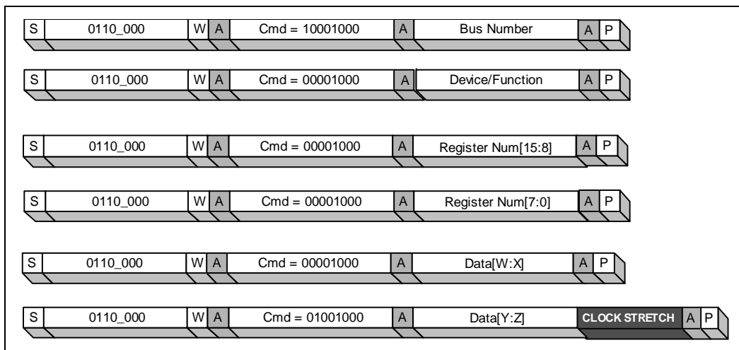
Figure 5-21. WORD Configuration Wrote Protocol (SMBus Byte Write, PEC Disabled)
