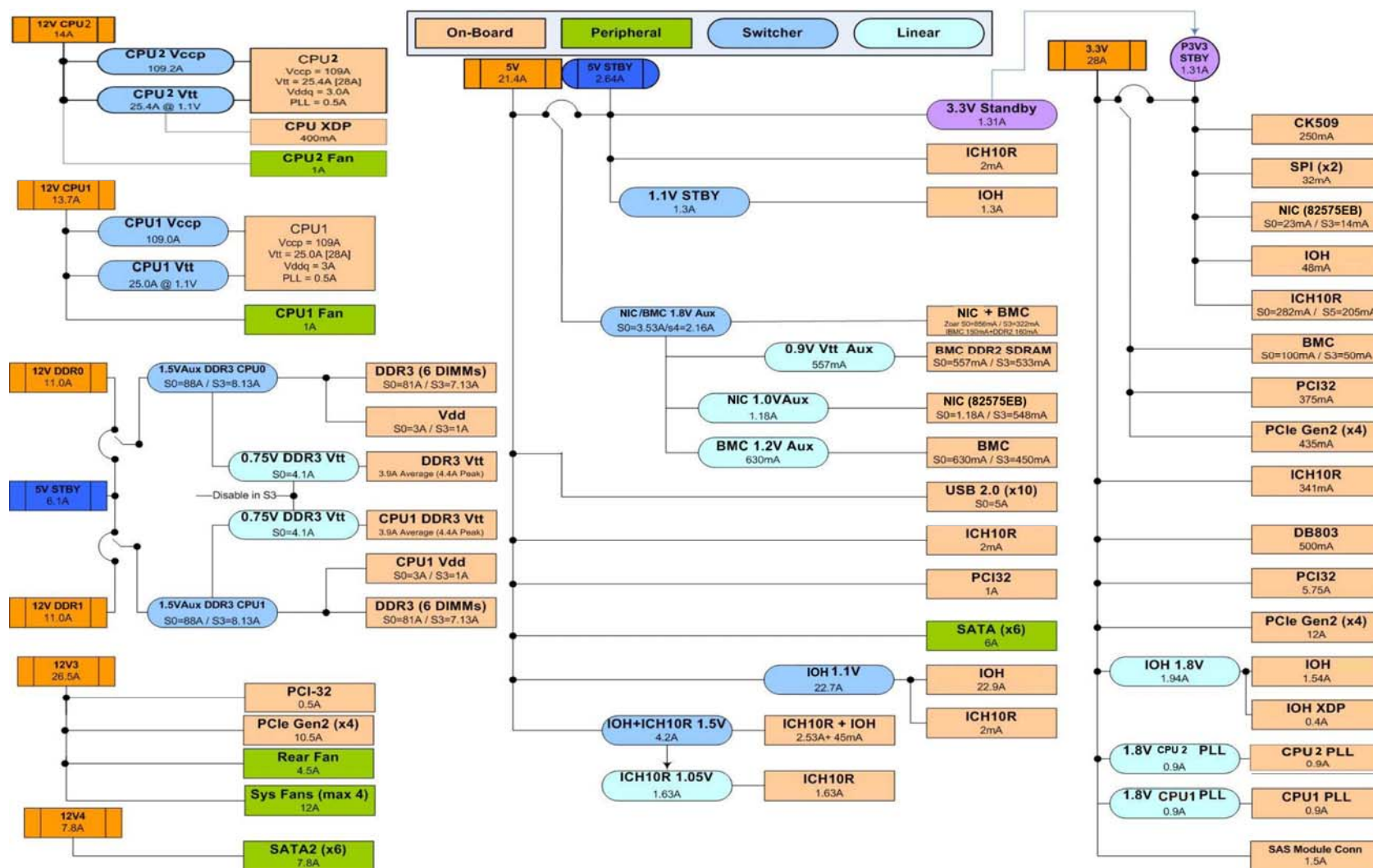
Figure 51. Power Distribution Block Diagram
