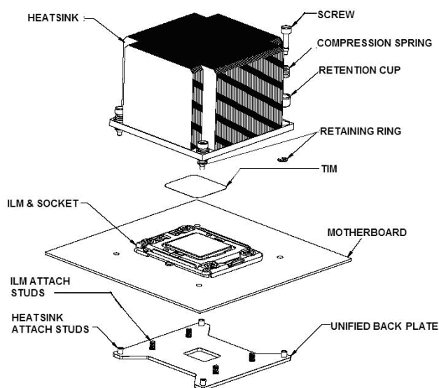
Figure 14. Unified Retention System and Unified Back Plate Assembly
