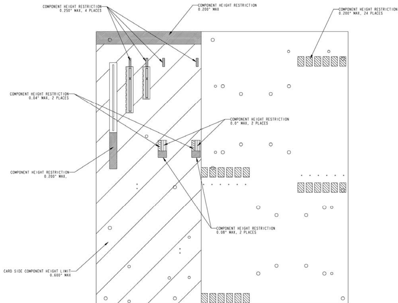
Figure 10. Intel® Workstation Board S5520SC – Primary Side Card-Side Keepout Zone
