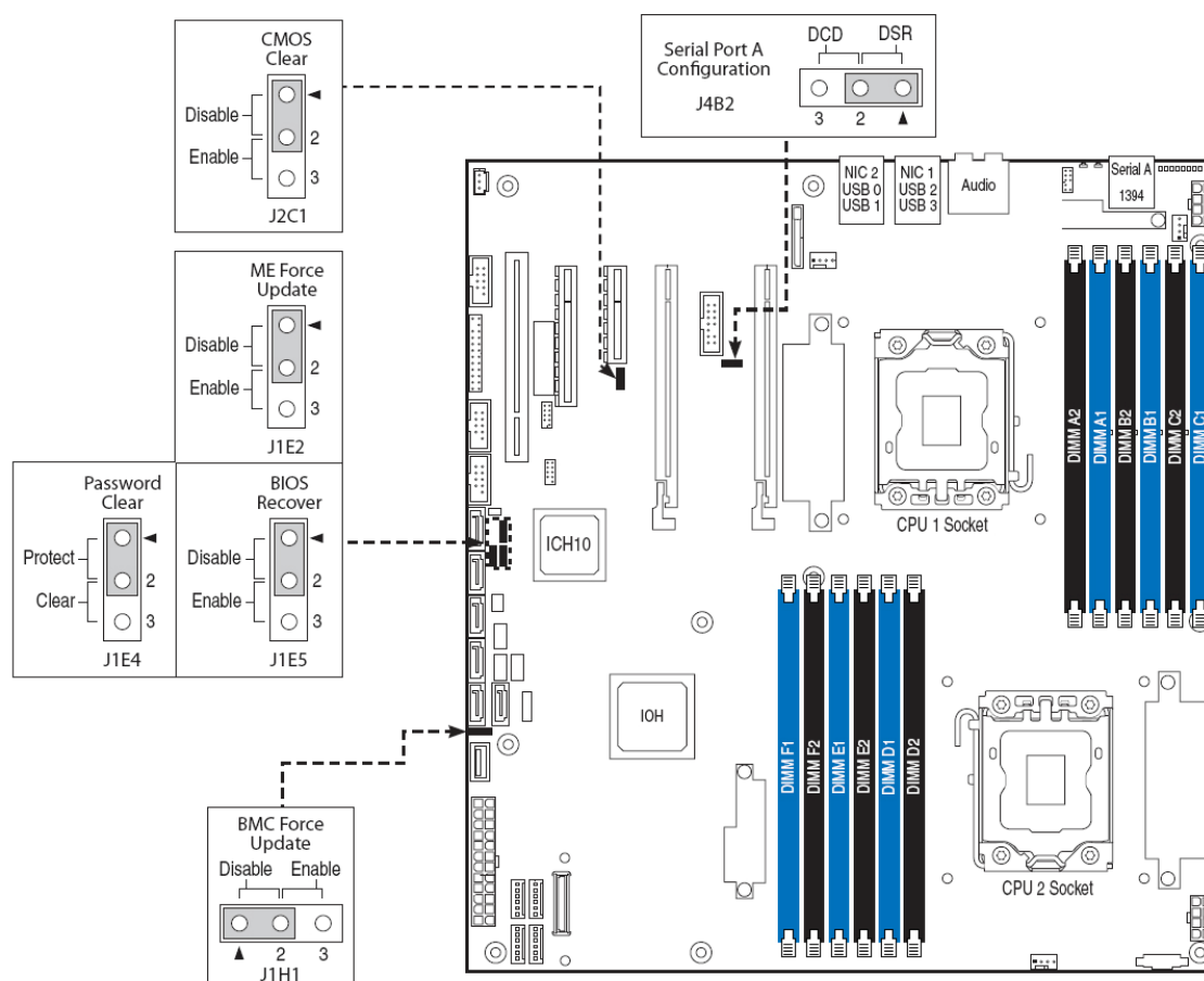
Figure 45. Jumper Blocks
