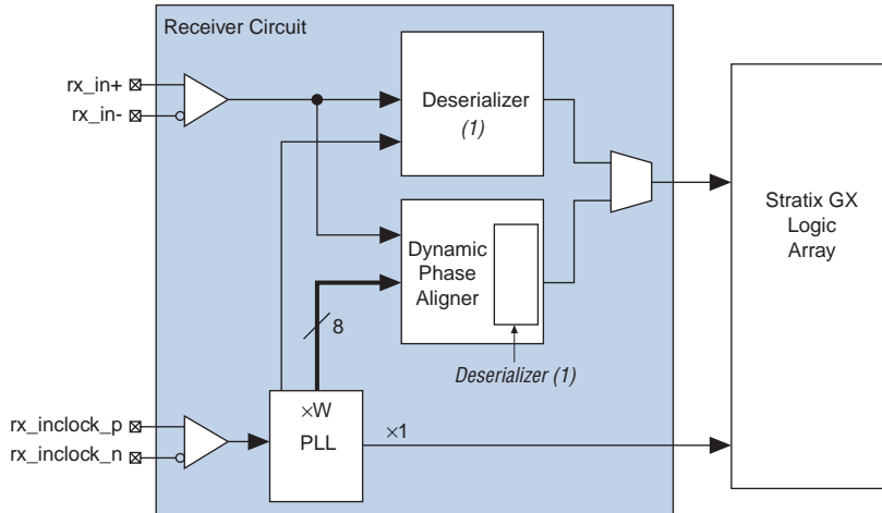
Figure 38. Source-Synchronous DPA Circuitry
