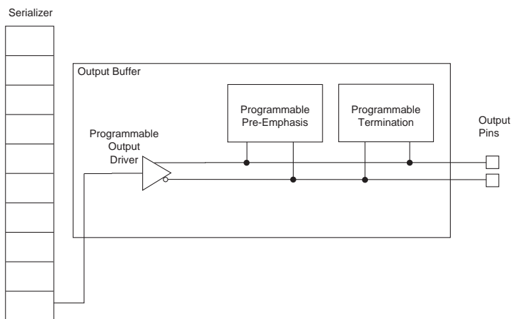
Figure 8. Output Buffer
