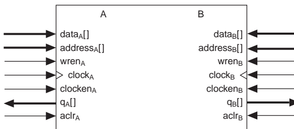
Figure 55. True Dual-Port Memory Configuration
