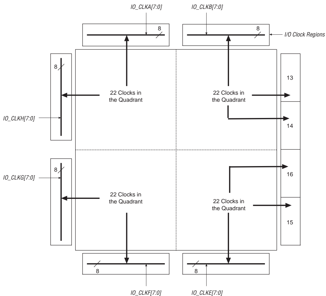
Figure 90. EP1SGX25 & EP1SGX10 Device I/O Clock Groups
