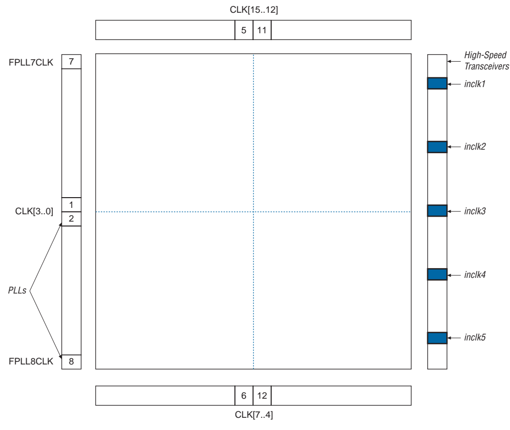
Figure 92. PLL Floorplan
