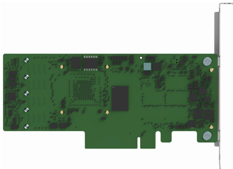
Figure 1 - Intel SAS RSP3TD160F RAID adapter Layout
