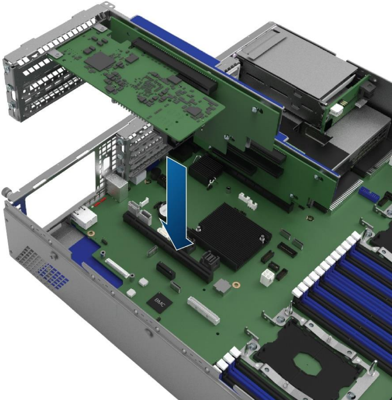
Figure 17 RAID Adapter Installation (insert riser card)
