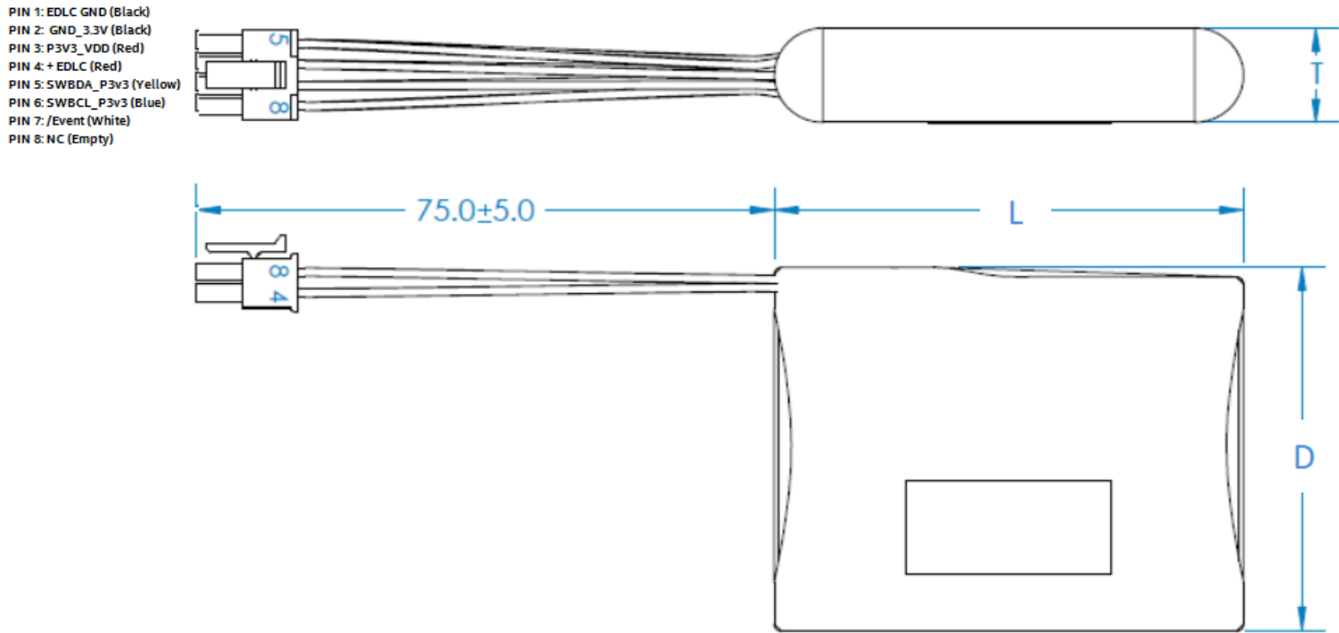
Figure 19. FBU345 layout
