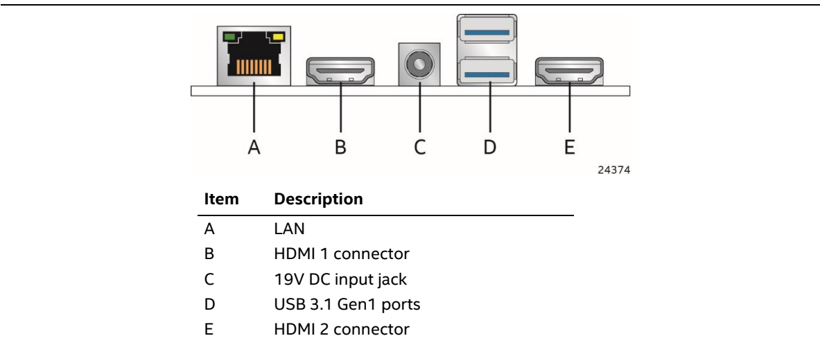
Figure 10. Back Panel Connectors
